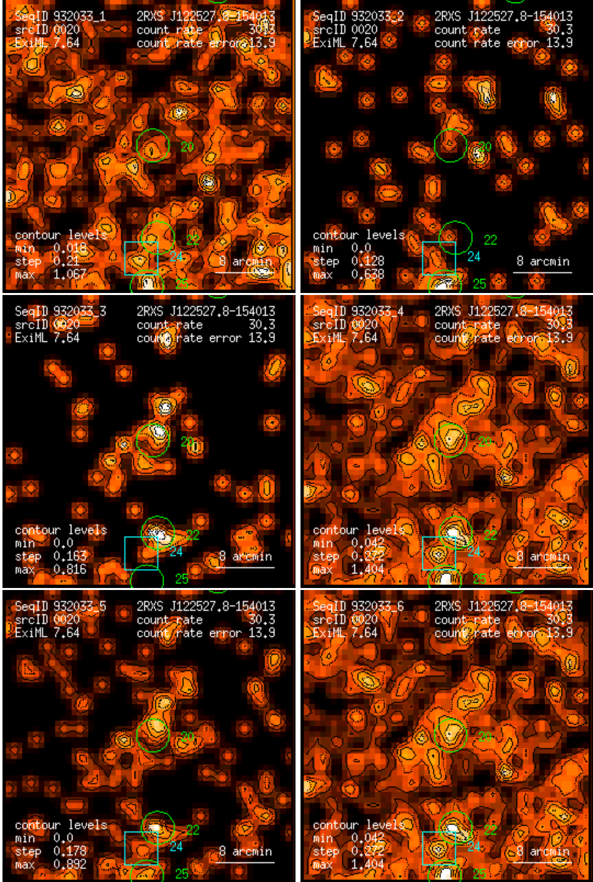
Figure 20: RASS 932033: detection 0020: band rate images, Gaussian filter: (1) PSPC channels 11 – 41, (2) 52 – 90, (3) 91 – 201, (4) 11 – 235, (5) 52 – 201, (6) 11 – 201. Broad band rates in counts/ks. Band rate contour levels in counts/ks/arcmin 2 .
