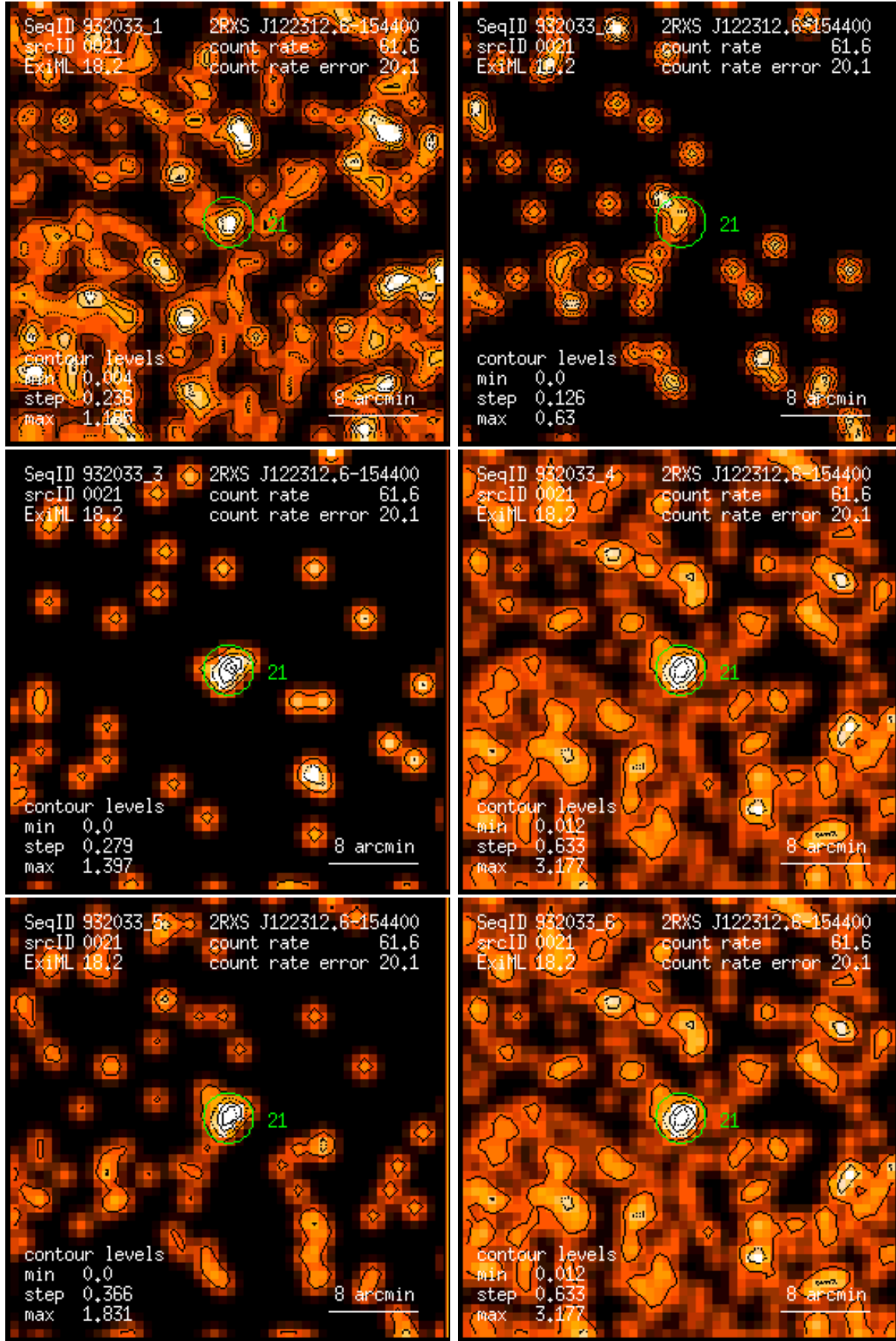
Figure 21: RASS 932033: detection 0021: band rate images, Gaussian filter: (1) PSPC channels 11 – 41, (2) 52 – 90, (3) 91 – 201, (4) 11 – 235, (5) 52 – 201, (6) 11 – 201. Broad band rates in counts/ks. Band rate contour levels in counts/ks/arcmin 2 .
