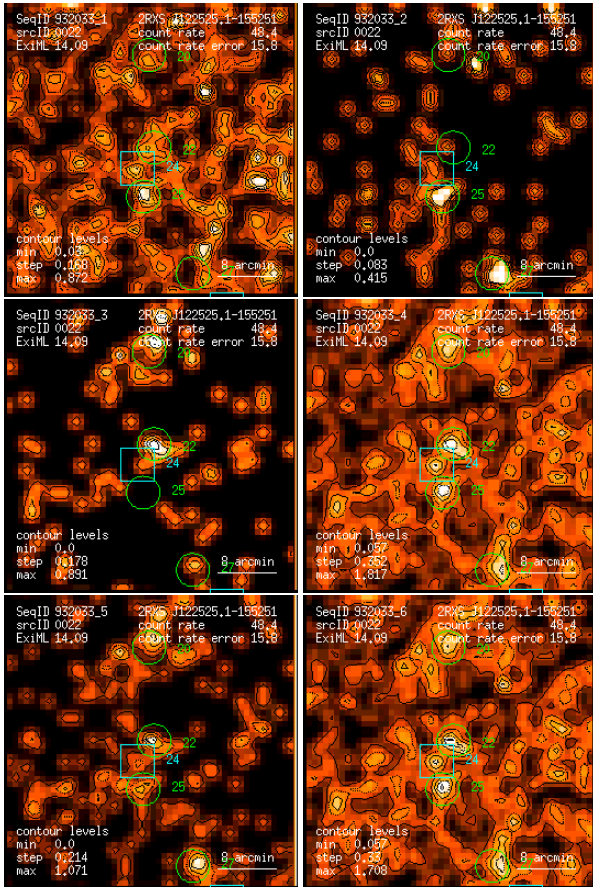
Figure 22: RASS 932033: detection 0022: band rate images, Gaussian filter: (1) PSPC channels 11 – 41, (2) 52 – 90, (3) 91 – 201, (4) 11 – 235, (5) 52 – 201, (6) 11 – 201. Broad band rates in counts/ks. Band rate contour levels in counts/ks/arcmin 2 .
