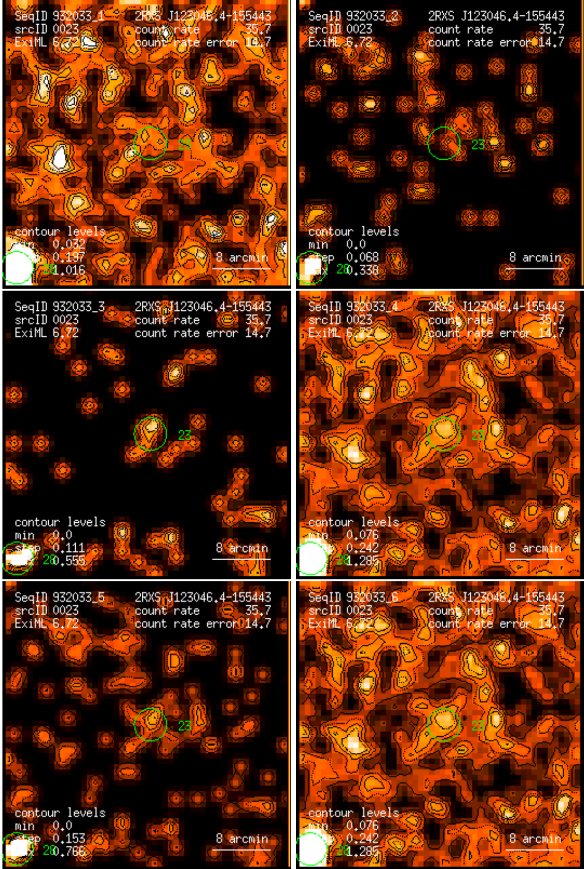
Figure 23: RASS 932033: detection 0023: band rate images, Gaussian filter: (1) PSPC channels 11 – 41, (2) 52 – 90, (3) 91 – 201, (4) 11 – 235, (5) 52 – 201, (6) 11 – 201. Broad band rates in counts/ks. Band rate contour levels in counts/ks/arcmin 2 .
