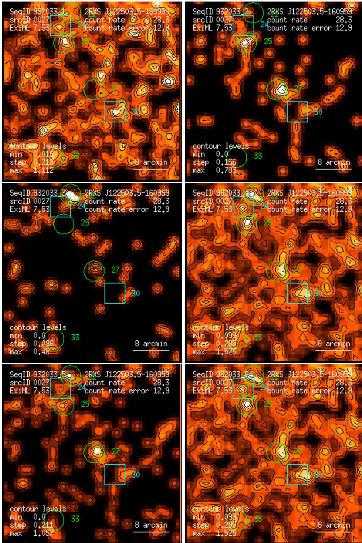
Figure 27: RASS 932033: detection 0027: band rate images, Gaussian filter: (1) PSPC channels 11 – 41, (2) 52 – 90, (3) 91 – 201, (4) 11 – 235, (5) 52 – 201, (6) 11 – 201. Broad band rates in counts/ks. Band rate contour levels in counts/ks/arcmin 2 .
