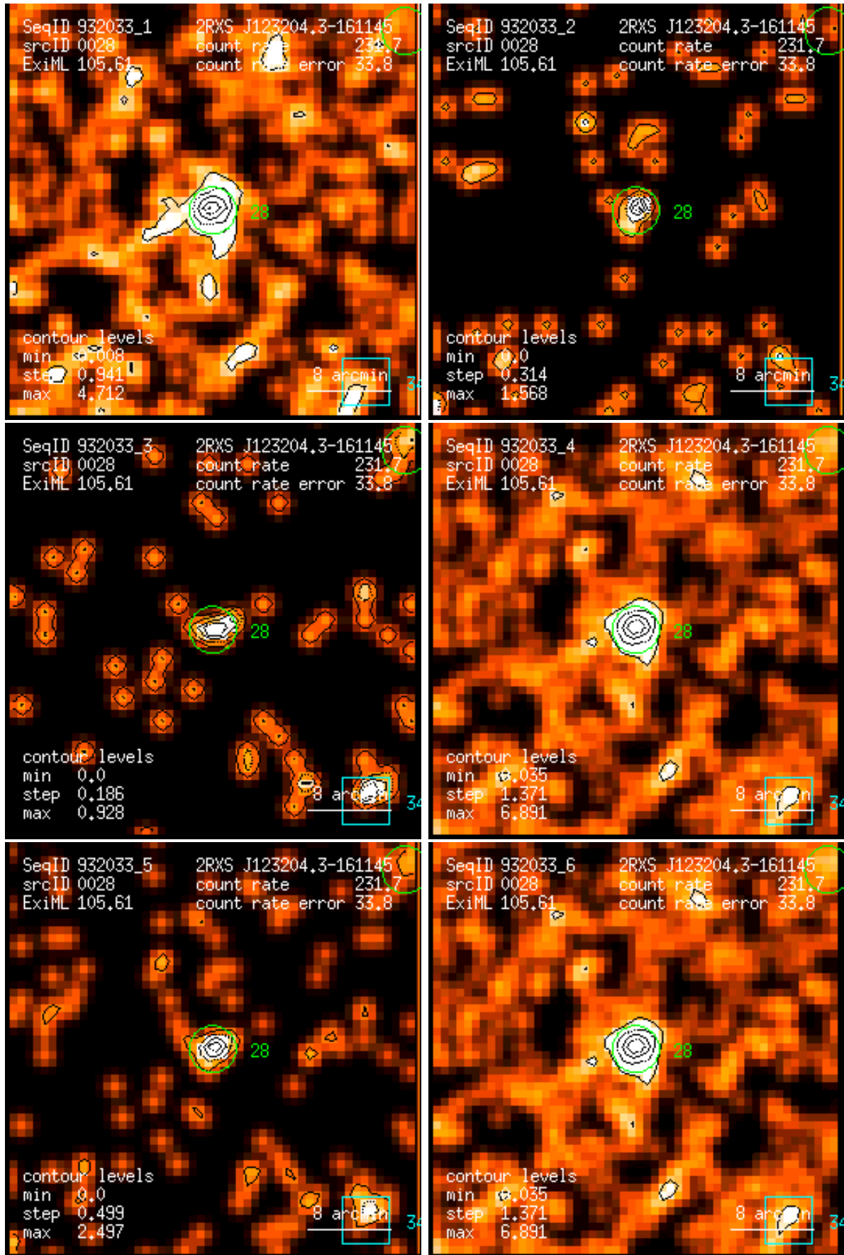
Figure 28: RASS 932033: detection 0028: band rate images, Gaussian filter: (1) PSPC channels 11 – 41, (2) 52 – 90, (3) 91 – 201, (4) 11 – 235, (5) 52 – 201, (6) 11 – 201. Broad band rates in counts/ks. Band rate contour levels in counts/ks/arcmin 2 .
