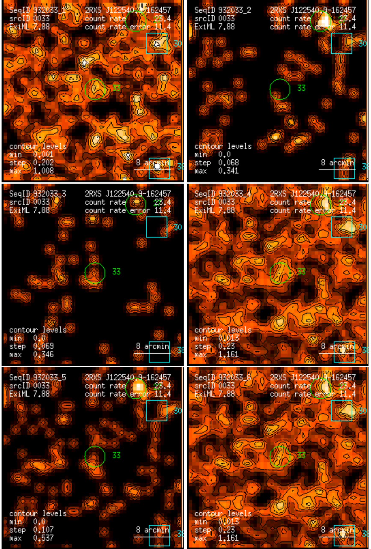
Figure 33: RASS 932033: detection 0033: band rate images, Gaussian filter: (1) PSPC channels 11 – 41, (2) 52 – 90, (3) 91 – 201, (4) 11 – 235, (5) 52 – 201, (6) 11 – 201. Broad band rates in counts/ks. Band rate contour levels in counts/ks/arcmin 2 .
