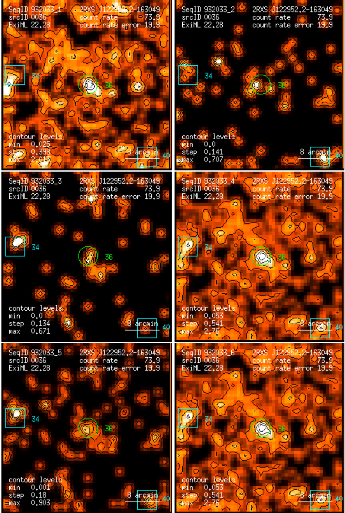
Figure 36: RASS 932033: detection 0036: band rate images, Gaussian filter: (1) PSPC channels 11 – 41, (2) 52 – 90, (3) 91 – 201, (4) 11 – 235, (5) 52 – 201, (6) 11 – 201. Broad band rates in counts/ks. Band rate contour levels in counts/ks/arcmin 2 .
