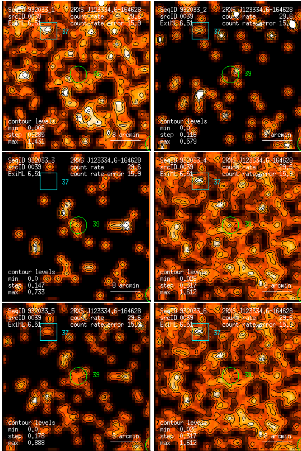
Figure 39: RASS 932033: detection 0039: band rate images, Gaussian filter: (1) PSPC channels 11 – 41, (2) 52 – 90, (3) 91 – 201, (4) 11 – 235, (5) 52 – 201, (6) 11 – 201. Broad band rates in counts/ks. Band rate contour levels in counts/ks/arcmin 2 .
