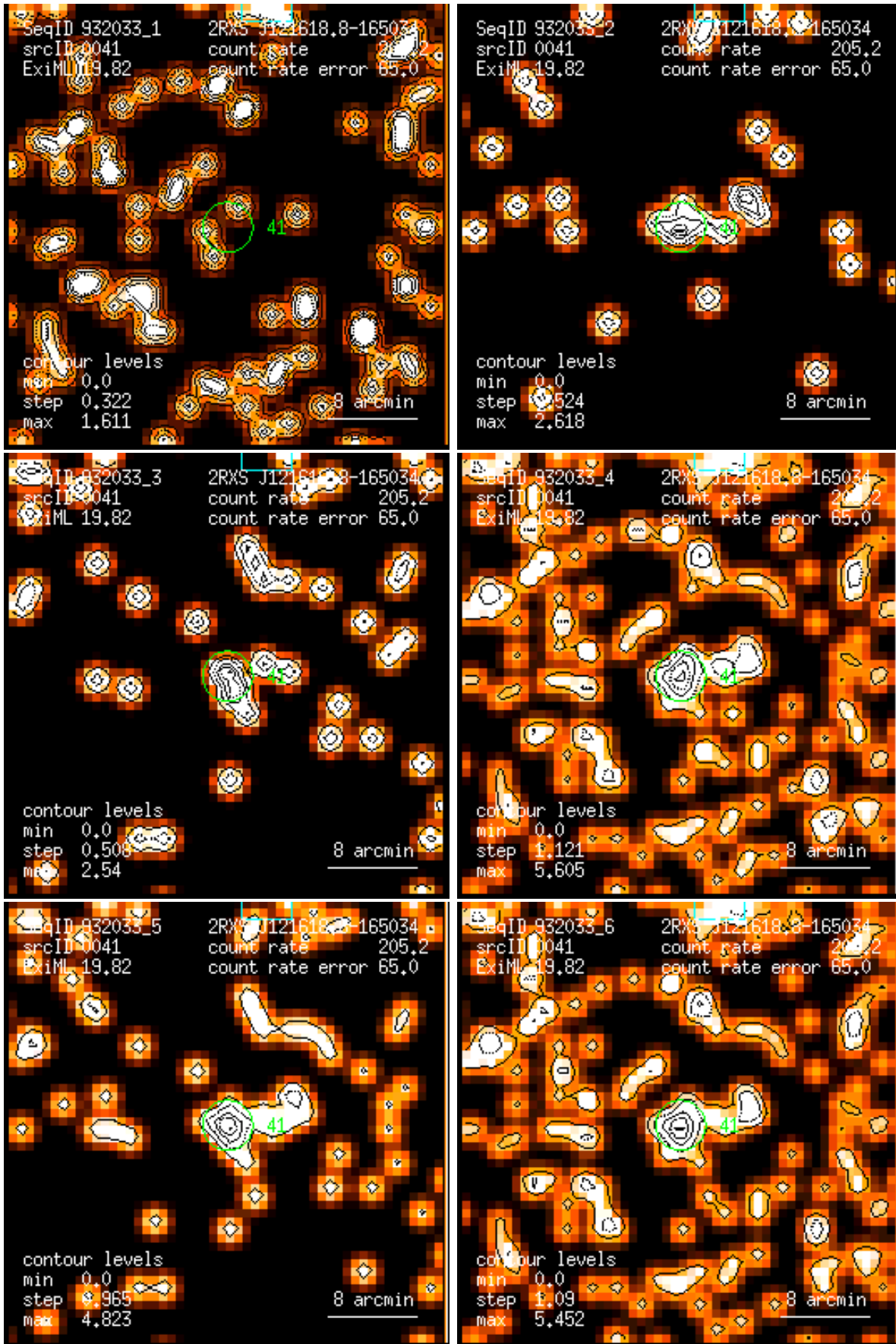
Figure 41: RASS 932033: detection 0041: band rate images, Gaussian filter: (1) PSPC channels 11 – 41, (2) 52 – 90, (3) 91 – 201, (4) 11 – 235, (5) 52 – 201, (6) 11 – 201. Broad band rates in counts/ks. Band rate contour levels in counts/ks/arcmin 2 .
