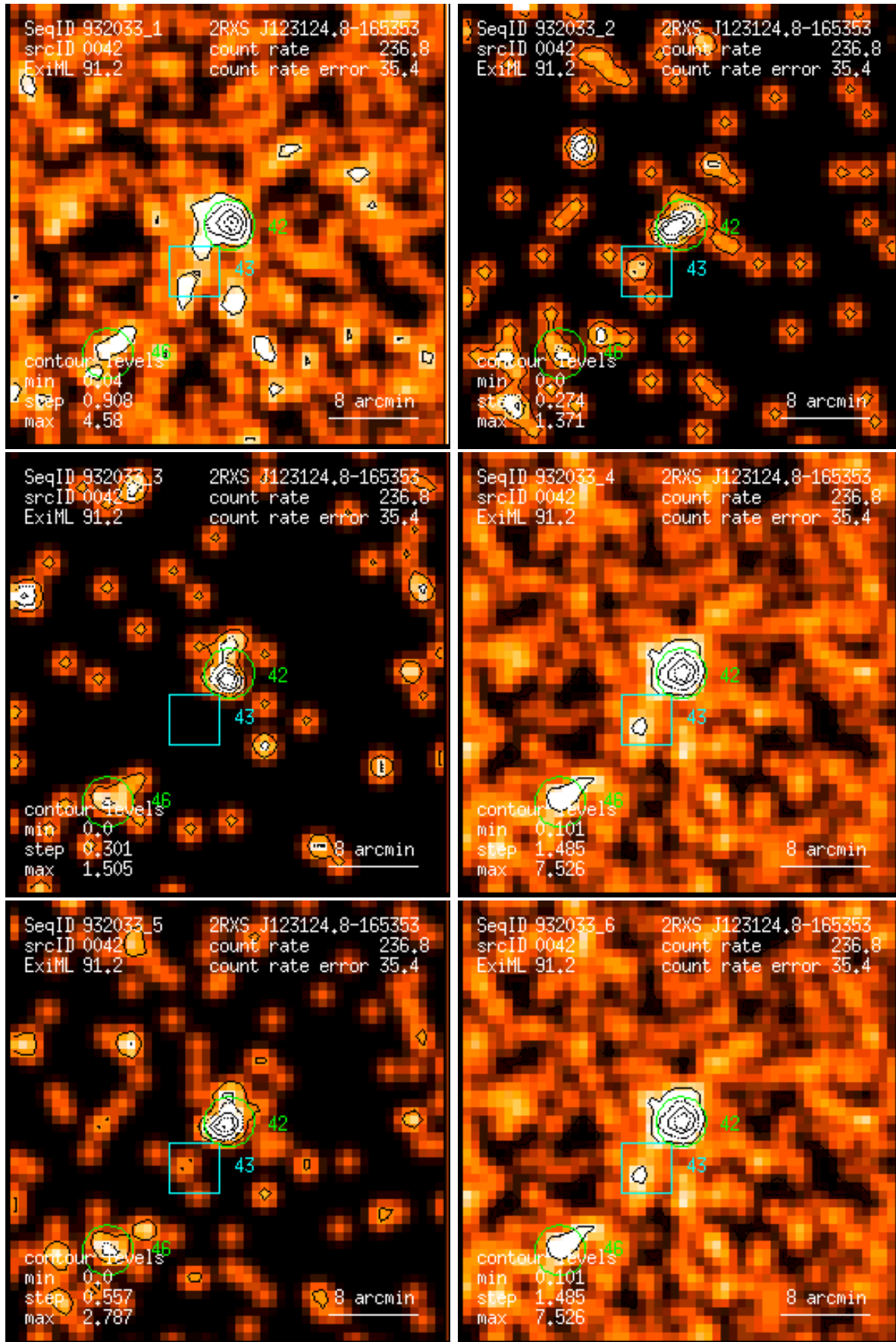
Figure 42: RASS 932033: detection 0042: band rate images, Gaussian filter: (1) PSPC channels 11 – 41, (2) 52 – 90, (3) 91 – 201, (4) 11 – 235, (5) 52 – 201, (6) 11 – 201. Broad band rates in counts/ks. Band rate contour levels in counts/ks/arcmin 2 .
