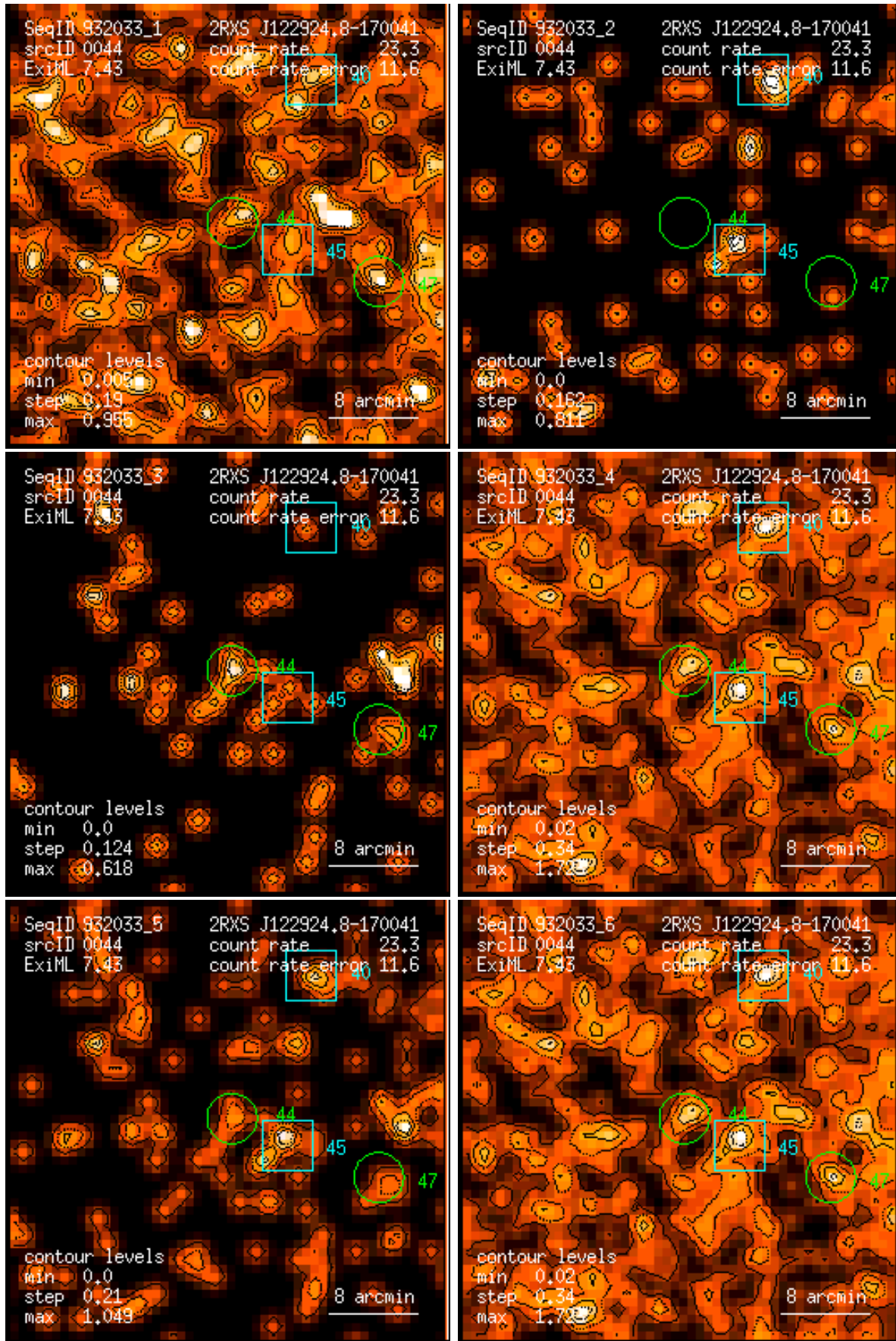
Figure 44: RASS 932033: detection 0044: band rate images, Gaussian filter: (1) PSPC channels 11 – 41, (2) 52 – 90, (3) 91 – 201, (4) 11 – 235, (5) 52 – 201, (6) 11 – 201. Broad band rates in counts/ks. Band rate contour levels in counts/ks/arcmin 2 .
