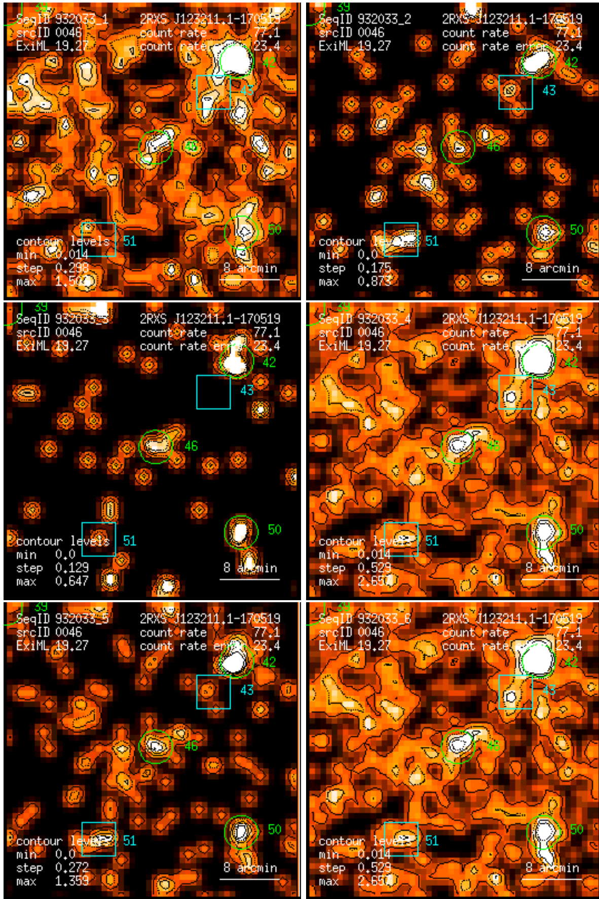
Figure 46: RASS 932033: detection 0046: band rate images, Gaussian filter: (1) PSPC channels 11 – 41, (2) 52 – 90, (3) 91 – 201, (4) 11 – 235, (5) 52 – 201, (6) 11 – 201. Broad band rates in counts/ks. Band rate contour levels in counts/ks/arcmin 2 .
