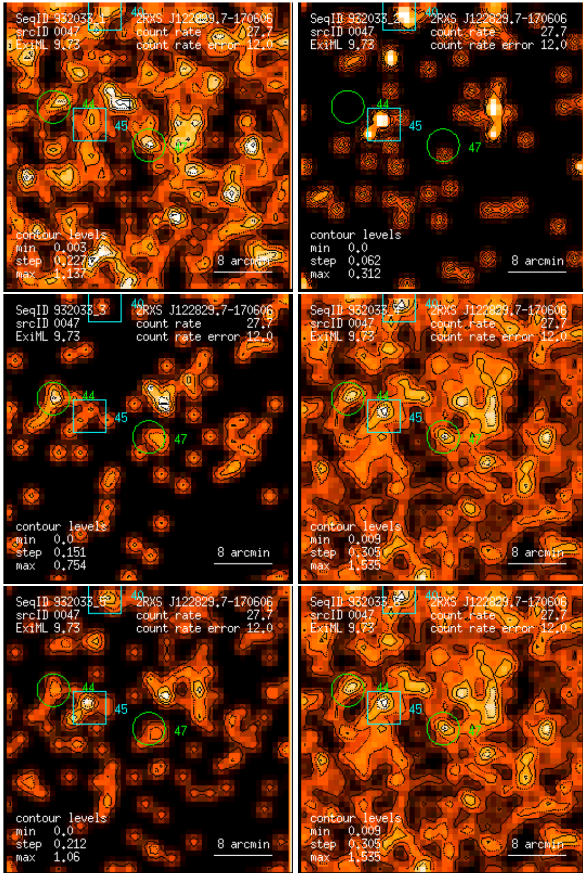
Figure 47: RASS 932033: detection 0047: band rate images, Gaussian filter: (1) PSPC channels 11 – 41, (2) 52 – 90, (3) 91 – 201, (4) 11 – 235, (5) 52 – 201, (6) 11 – 201. Broad band rates in counts/ks. Band rate contour levels in counts/ks/arcmin 2 .
