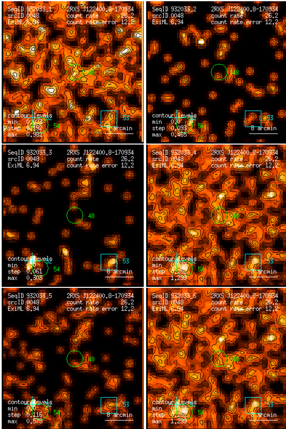
Figure 48: RASS 932033: detection 0048: band rate images, Gaussian filter: (1) PSPC channels 11 – 41, (2) 52 – 90, (3) 91 – 201, (4) 11 – 235, (5) 52 – 201, (6) 11 – 201. Broad band rates in counts/ks. Band rate contour levels in counts/ks/arcmin 2 .
