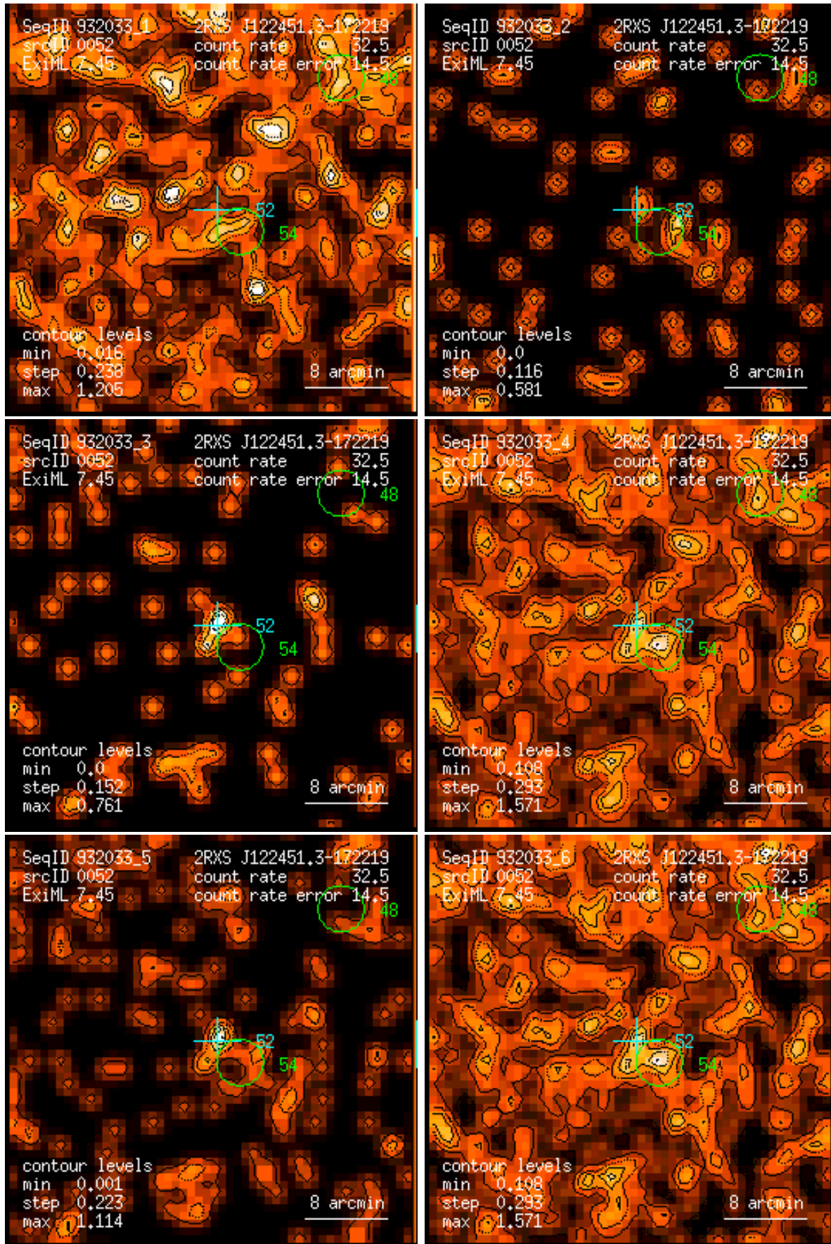
Figure 52: RASS 932033: detection 0052: band rate images, Gaussian filter: (1) PSPC channels 11 – 41, (2) 52 – 90, (3) 91 – 201, (4) 11 – 235, (5) 52 – 201, (6) 11 – 201. Broad band rates in counts/ks. Band rate contour levels in counts/ks/arcmin 2 .
