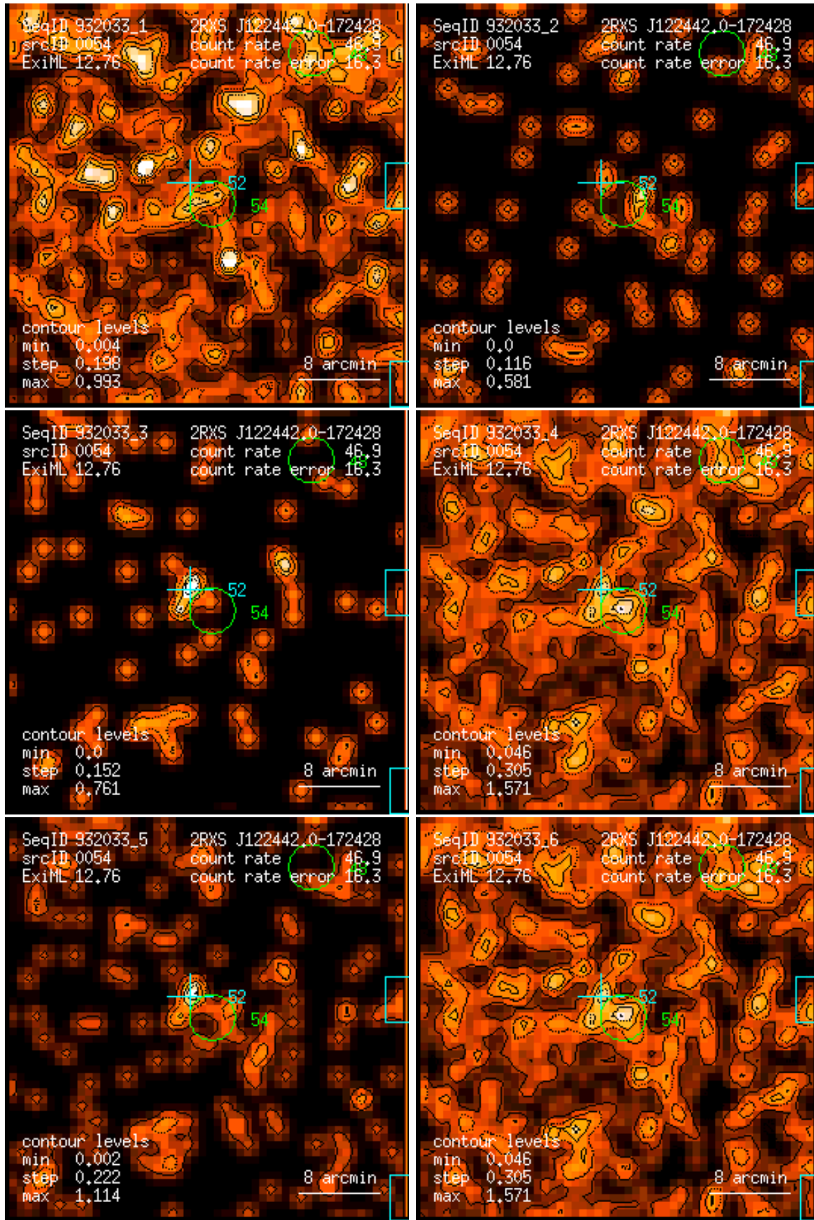
Figure 54: RASS 932033: detection 0054: band rate images, Gaussian filter: (1) PSPC channels 11 – 41, (2) 52 – 90, (3) 91 – 201, (4) 11 – 235, (5) 52 – 201, (6) 11 – 201. Broad band rates in counts/ks. Band rate contour levels in counts/ks/arcmin 2 .
