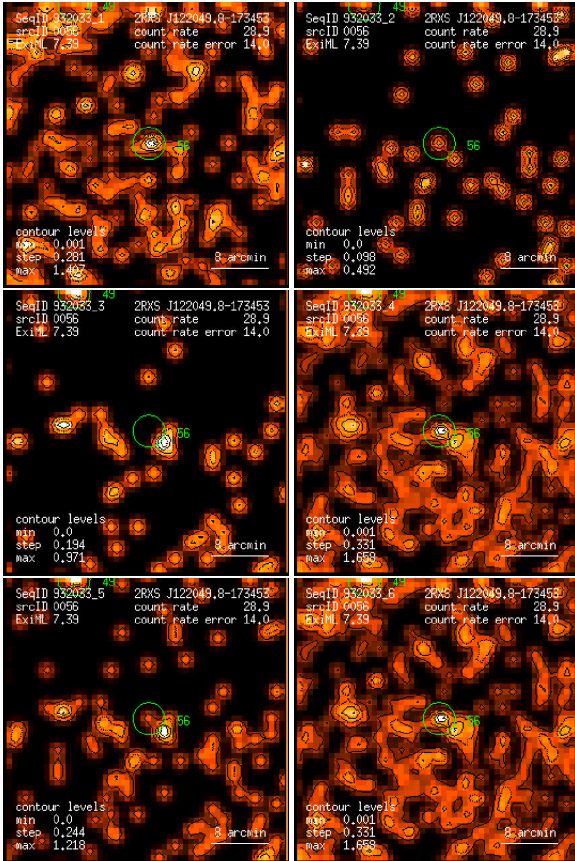
Figure 56: RASS 932033: detection 0056: band rate images, Gaussian filter: (1) PSPC channels 11 – 41, (2) 52 – 90, (3) 91 – 201, (4) 11 – 235, (5) 52 – 201, (6) 11 – 201. Broad band rates in counts/ks. Band rate contour levels in counts/ks/arcmin 2 .
