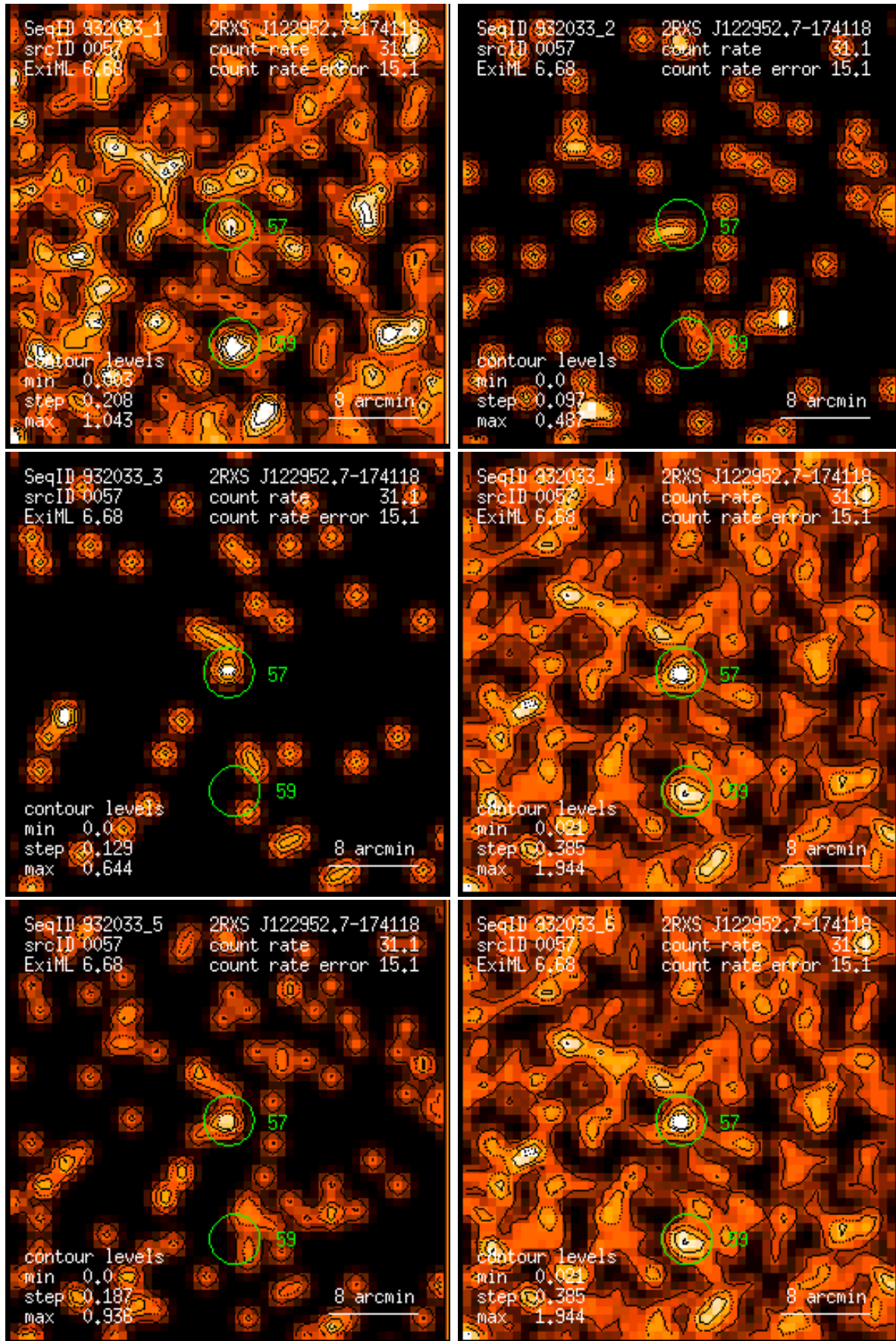
Figure 57: RASS 932033: detection 0057: band rate images, Gaussian filter: (1) PSPC channels 11 – 41, (2) 52 – 90, (3) 91 – 201, (4) 11 – 235, (5) 52 – 201, (6) 11 – 201. Broad band rates in counts/ks. Band rate contour levels in counts/ks/arcmin 2 .
