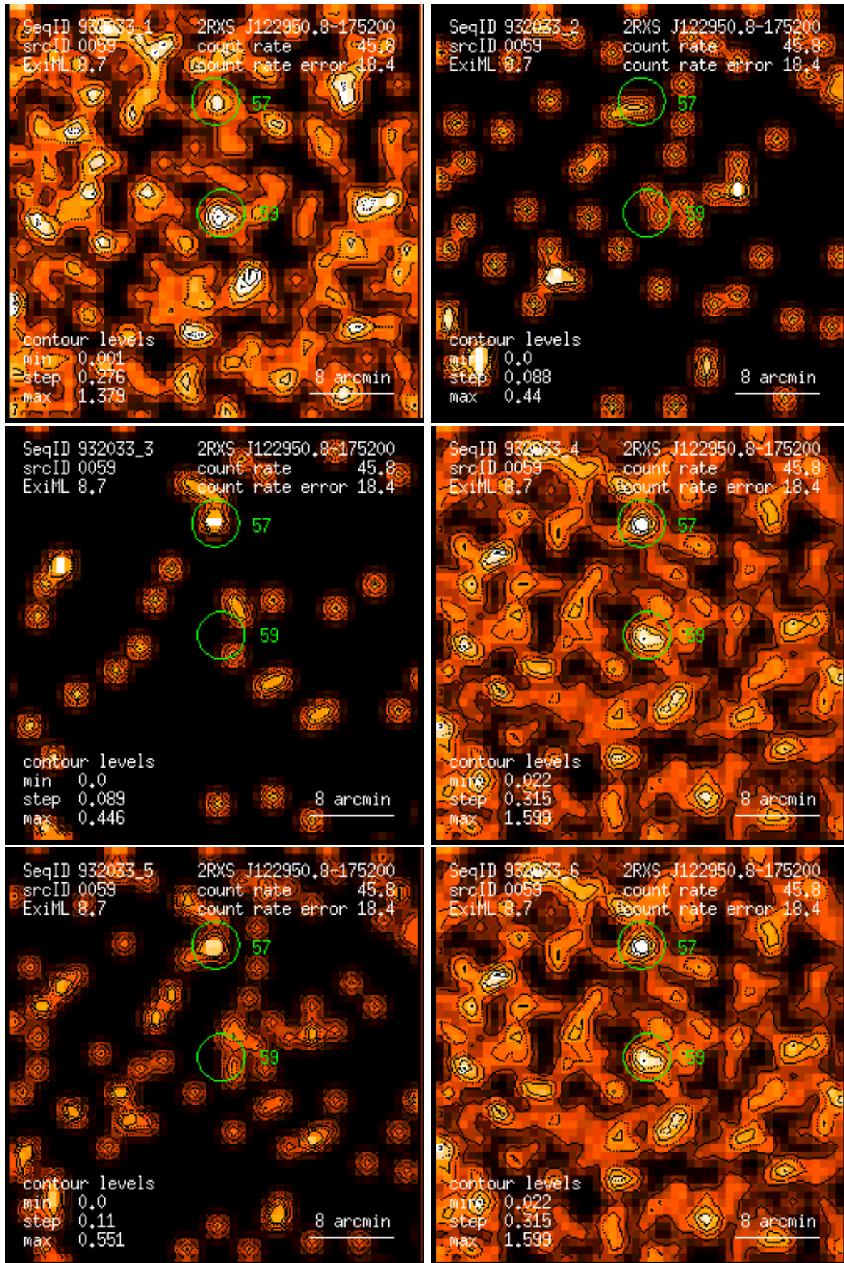
Figure 59: RASS 932033: detection 0059: band rate images, Gaussian filter: (1) PSPC channels 11 – 41, (2) 52 – 90, (3) 91 – 201, (4) 11 – 235, (5) 52 – 201, (6) 11 – 201. Broad band rates in counts/ks. Band rate contour levels in counts/ks/arcmin 2 .
