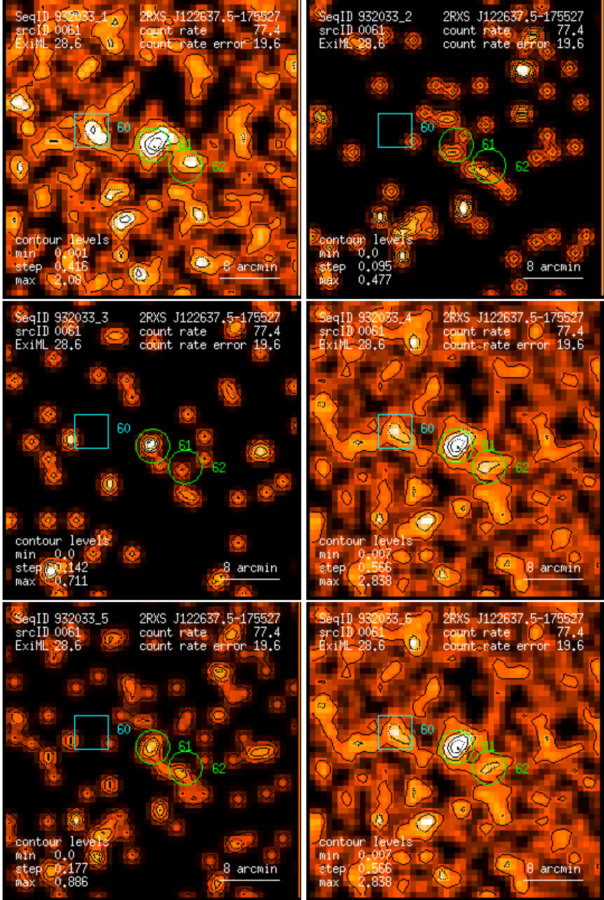
Figure 61: RASS 932033: detection 0061: band rate images, Gaussian filter: (1) PSPC channels 11 – 41, (2) 52 – 90, (3) 91 – 201, (4) 11 – 235, (5) 52 – 201, (6) 11 – 201. Broad band rates in counts/ks. Band rate contour levels in counts/ks/arcmin 2 .
