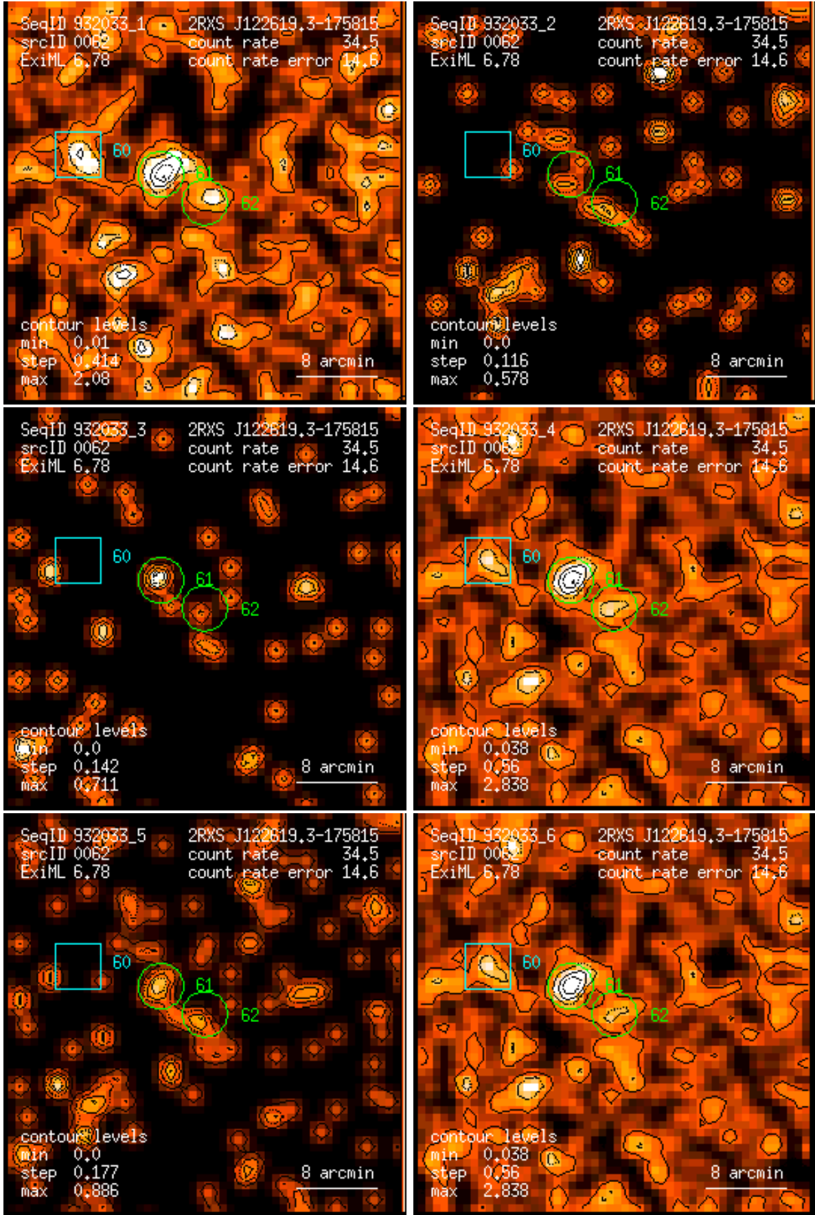
Figure 62: RASS 932033: detection 0062: band rate images, Gaussian filter: (1) PSPC channels 11 – 41, (2) 52 – 90, (3) 91 – 201, (4) 11 – 235, (5) 52 – 201, (6) 11 – 201. Broad band rates in counts/ks. Band rate contour levels in counts/ks/arcmin 2 .
