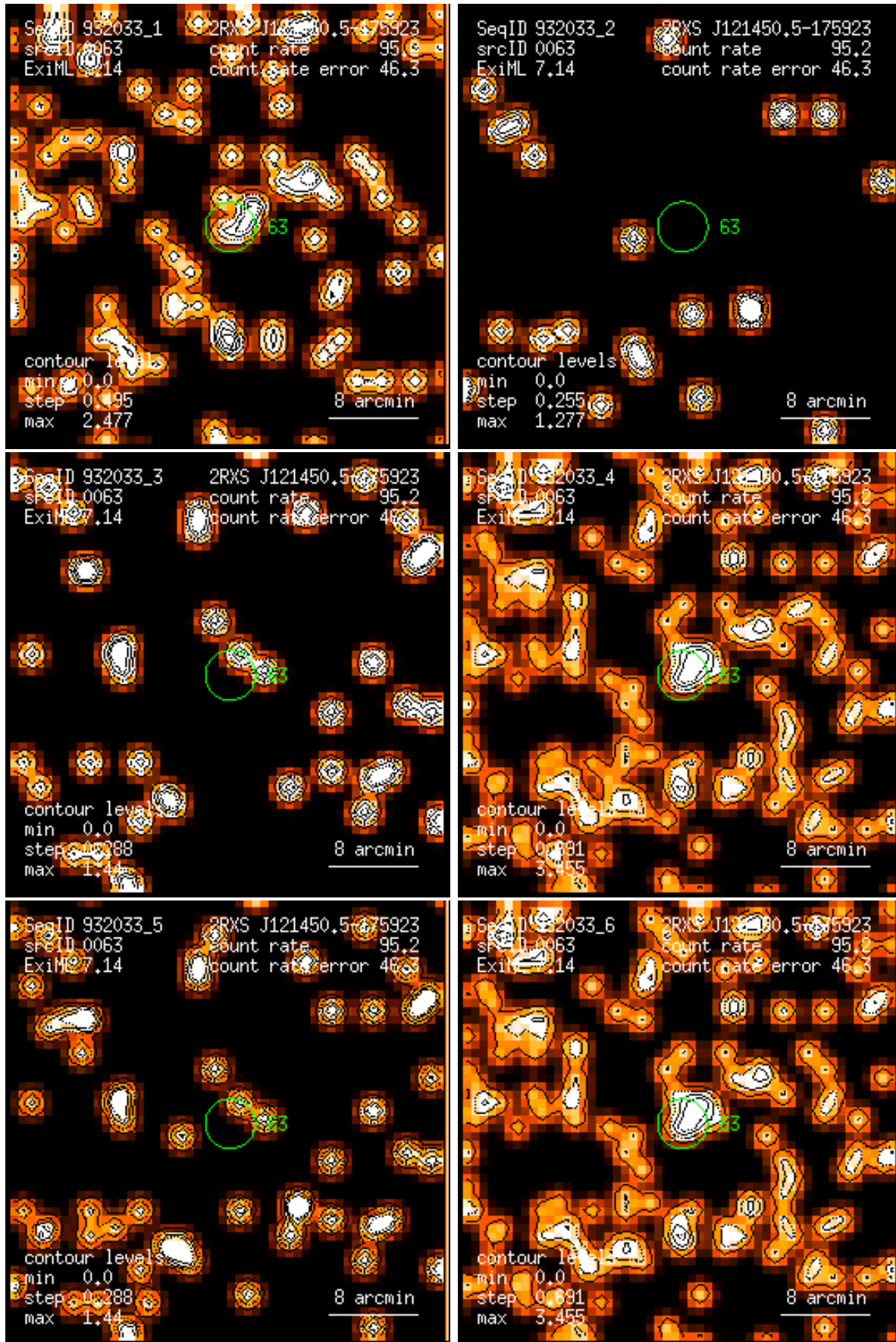
Figure 63: RASS 932033: detection 0063: band rate images, Gaussian filter: (1) PSPC channels 11 – 41, (2) 52 – 90, (3) 91 – 201, (4) 11 – 235, (5) 52 – 201, (6) 11 – 201. Broad band rates in counts/ks. Band rate contour levels in counts/ks/arcmin 2 .
