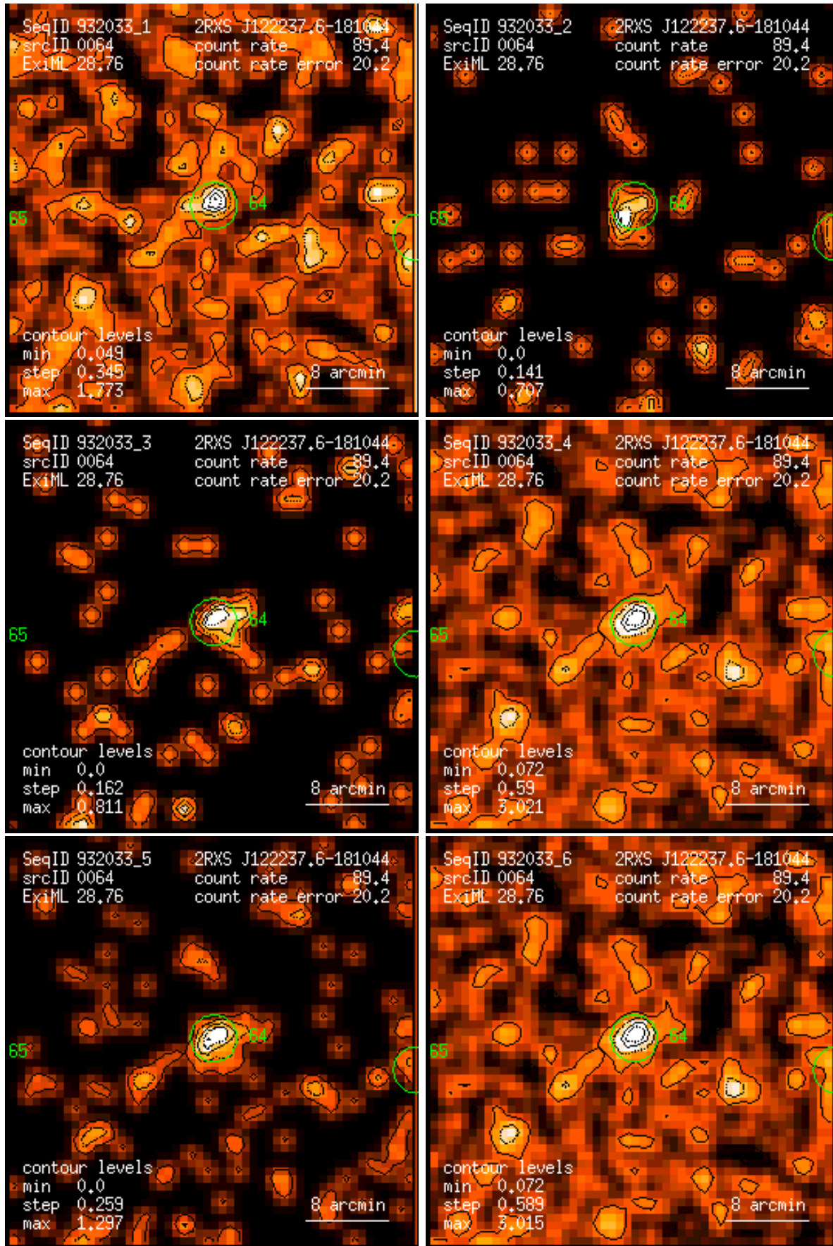
Figure 64: RASS 932033: detection 0064: band rate images, Gaussian filter: (1) PSPC channels 11 – 41, (2) 52 – 90, (3) 91 – 201, (4) 11 – 235, (5) 52 – 201, (6) 11 – 201. Broad band rates in counts/ks. Band rate contour levels in counts/ks/arcmin 2 .
