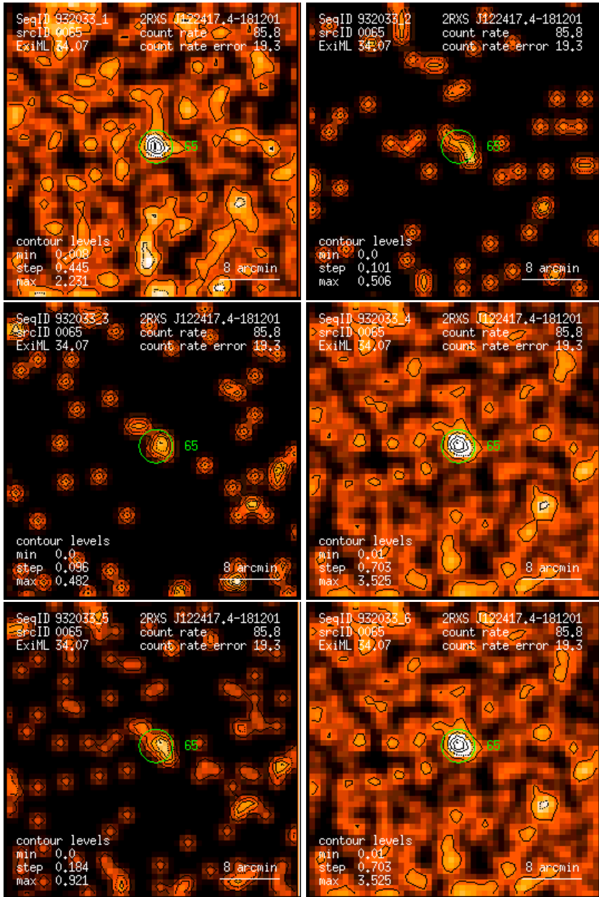
Figure 65: RASS 932033: detection 0065: band rate images, Gaussian filter: (1) PSPC channels 11 – 41, (2) 52 – 90, (3) 91 – 201, (4) 11 – 235, (5) 52 – 201, (6) 11 – 201. Broad band rates in counts/ks. Band rate contour levels in counts/ks/arcmin 2 .
