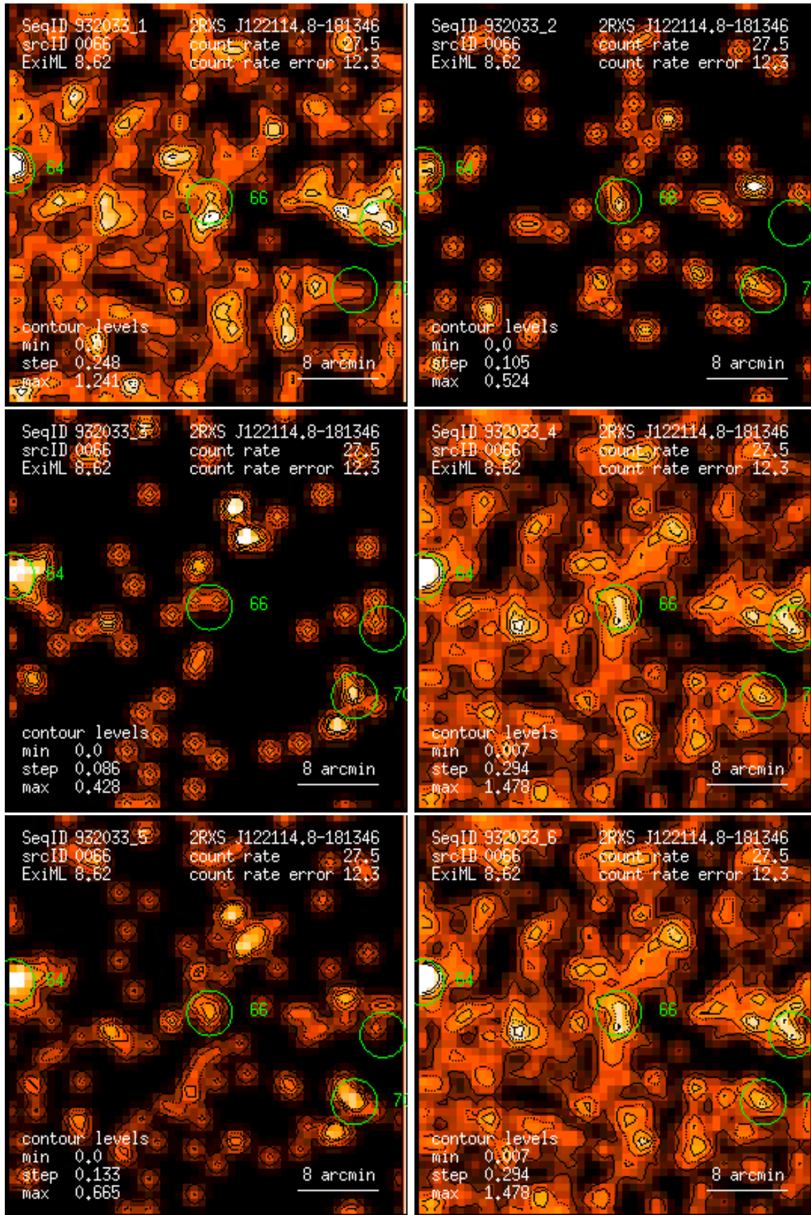
Figure 66: RASS 932033: detection 0066: band rate images, Gaussian filter: (1) PSPC channels 11 – 41, (2) 52 – 90, (3) 91 – 201, (4) 11 – 235, (5) 52 – 201, (6) 11 – 201. Broad band rates in counts/ks. Band rate contour levels in counts/ks/arcmin 2 .
