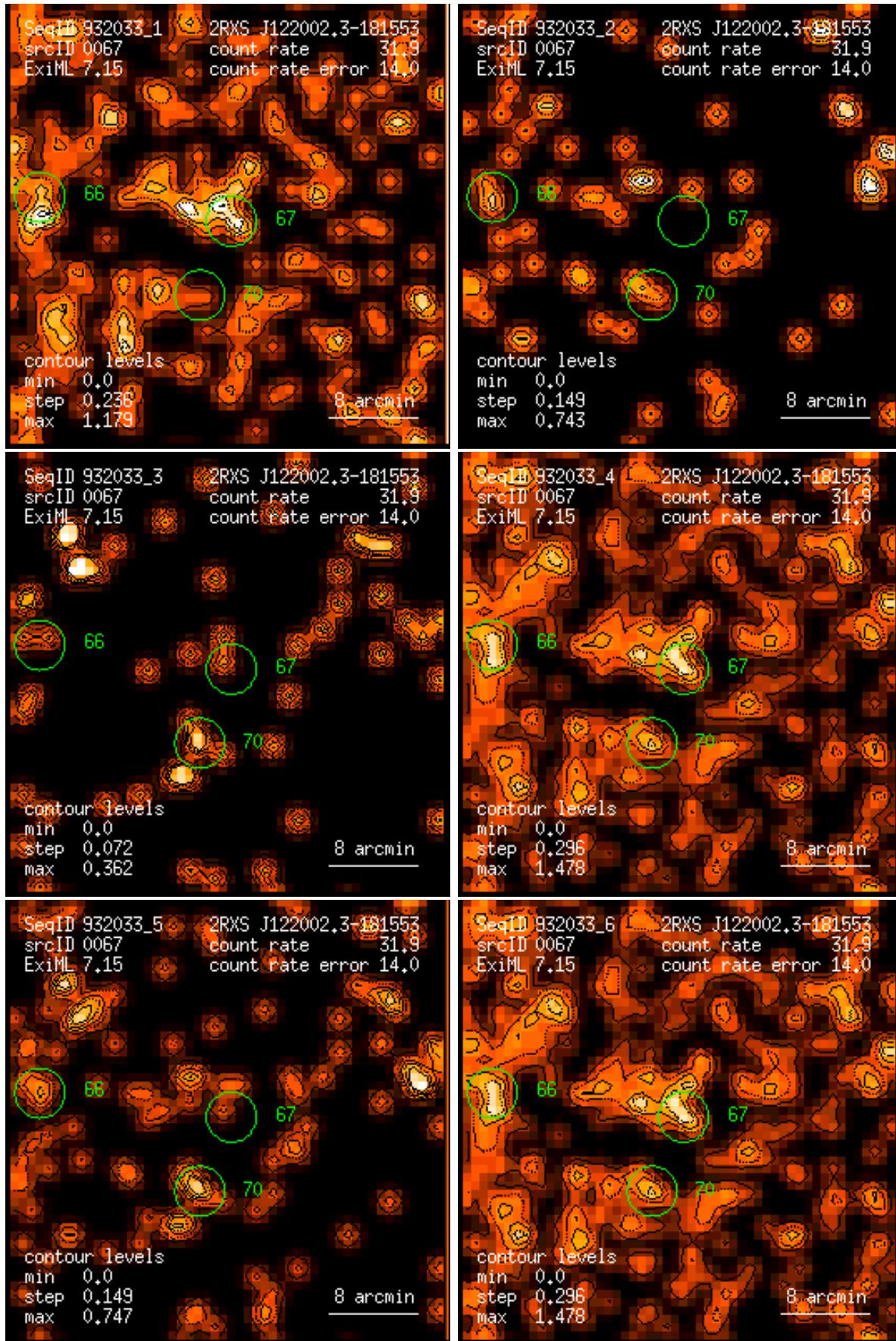
Figure 67: RASS 932033: detection 0067: band rate images, Gaussian filter: (1) PSPC channels 11 – 41, (2) 52 – 90, (3) 91 – 201, (4) 11 – 235, (5) 52 – 201, (6) 11 – 201. Broad band rates in counts/ks. Band rate contour levels in counts/ks/arcmin 2 .
