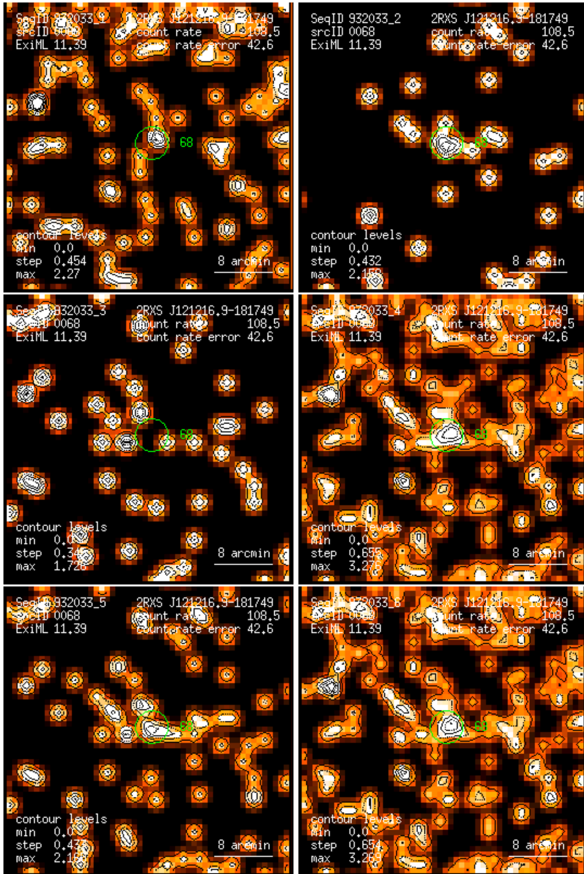
Figure 68: RASS 932033: detection 0068: band rate images, Gaussian filter: (1) PSPC channels 11 – 41, (2) 52 – 90, (3) 91 – 201, (4) 11 – 235, (5) 52 – 201, (6) 11 – 201. Broad band rates in counts/ks. Band rate contour levels in counts/ks/arcmin 2 .
