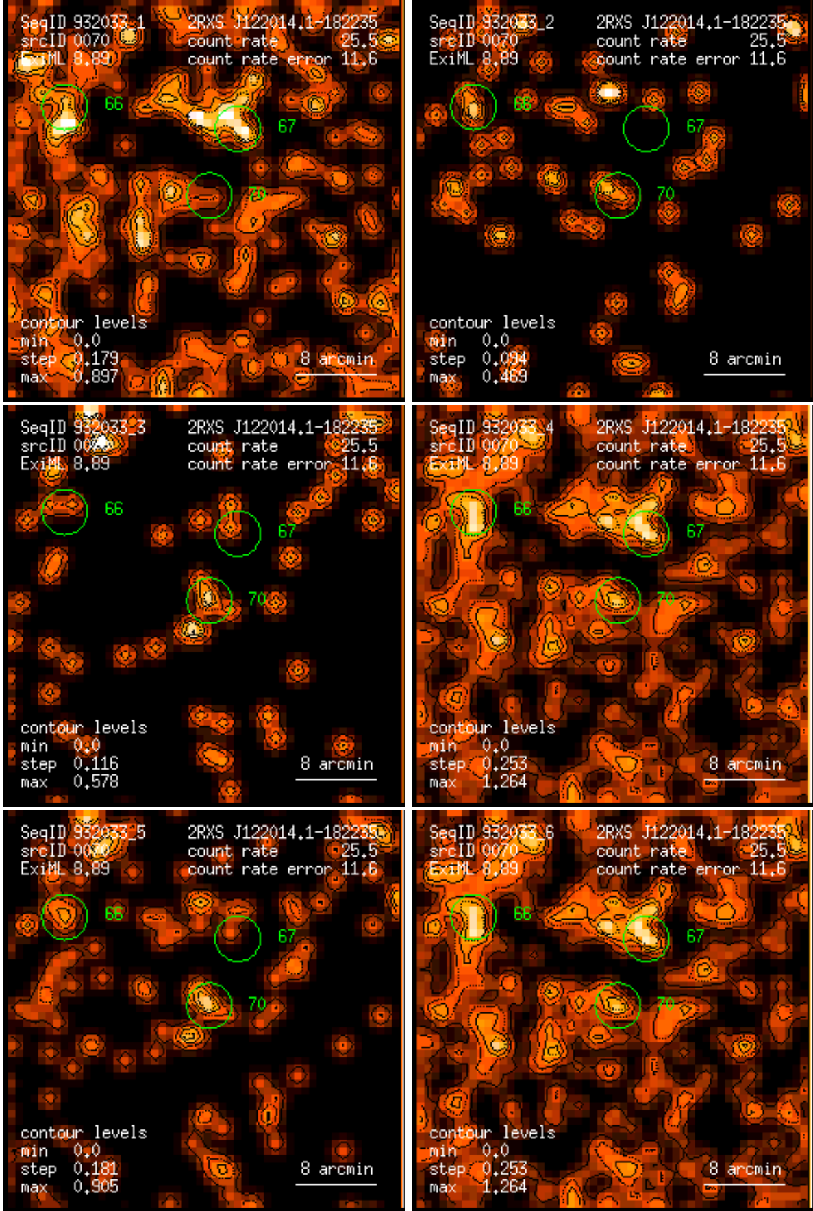
Figure 70: RASS 932033: detection 0070: band rate images, Gaussian filter: (1) PSPC channels 11 – 41, (2) 52 – 90, (3) 91 – 201, (4) 11 – 235, (5) 52 – 201, (6) 11 – 201. Broad band rates in counts/ks. Band rate contour levels in counts/ks/arcmin 2 .
