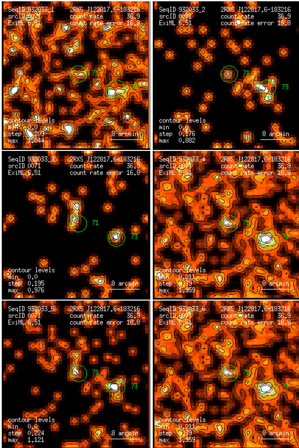
Figure 71: RASS 932033: detection 0071: band rate images, Gaussian filter: (1) PSPC channels 11 – 41, (2) 52 – 90, (3) 91 – 201, (4) 11 – 235, (5) 52 – 201, (6) 11 – 201. Broad band rates in counts/ks. Band rate contour levels in counts/ks/arcmin 2 .
