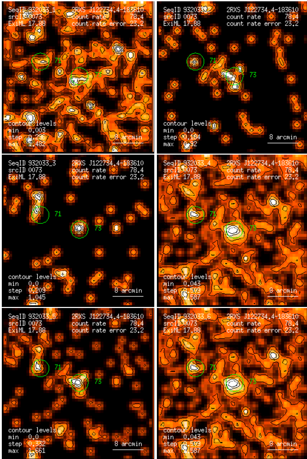
Figure 73: RASS 932033: detection 0073: band rate images, Gaussian filter: (1) PSPC channels 11 – 41, (2) 52 – 90, (3) 91 – 201, (4) 11 – 235, (5) 52 – 201, (6) 11 – 201. Broad band rates in counts/ks. Band rate contour levels in counts/ks/arcmin 2 .
