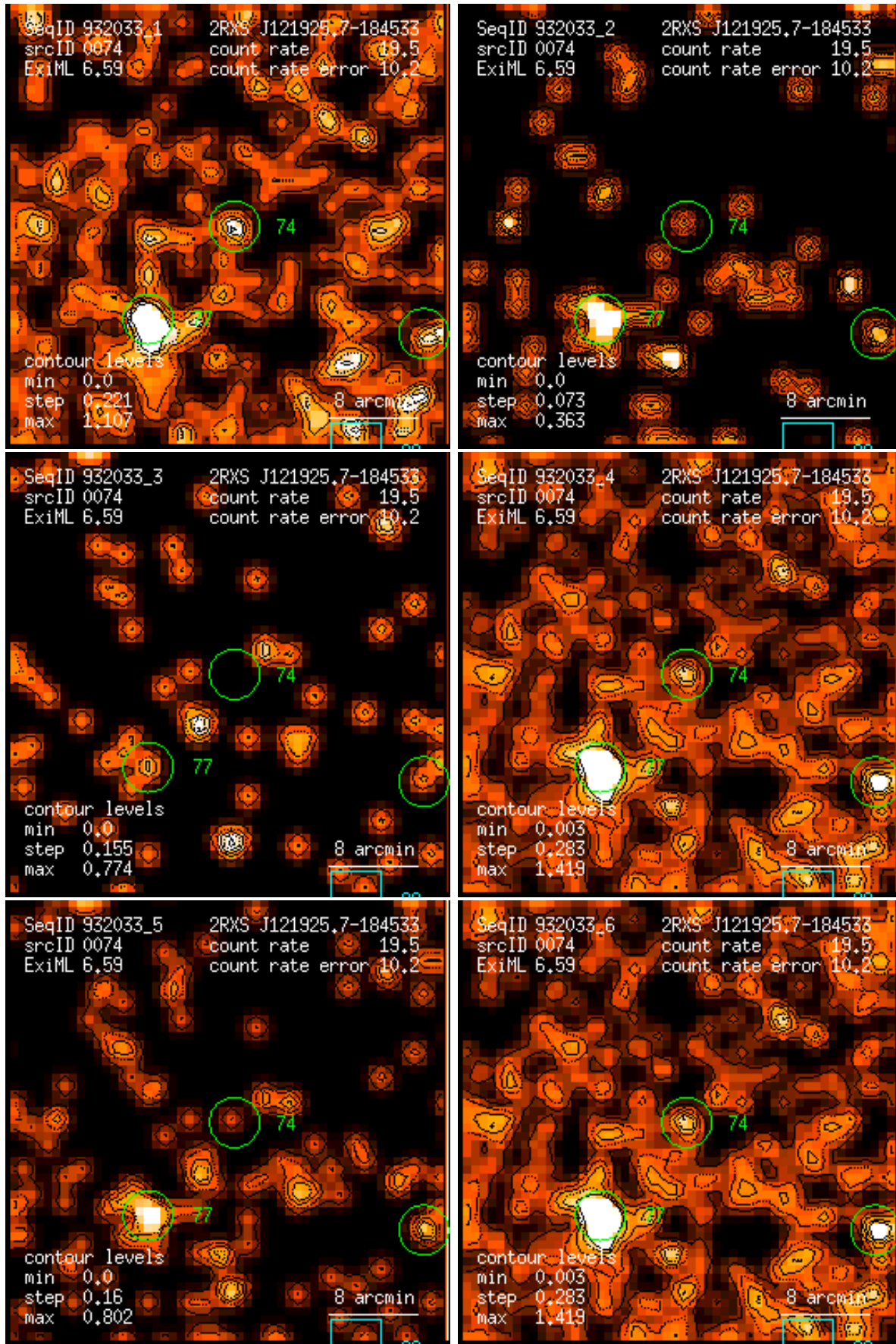
Figure 74: RASS 932033: detection 0074: band rate images, Gaussian filter: (1) PSPC channels 11 – 41, (2) 52 – 90, (3) 91 – 201, (4) 11 – 235, (5) 52 – 201, (6) 11 – 201. Broad band rates in counts/ks. Band rate contour levels in counts/ks/arcmin 2 .
