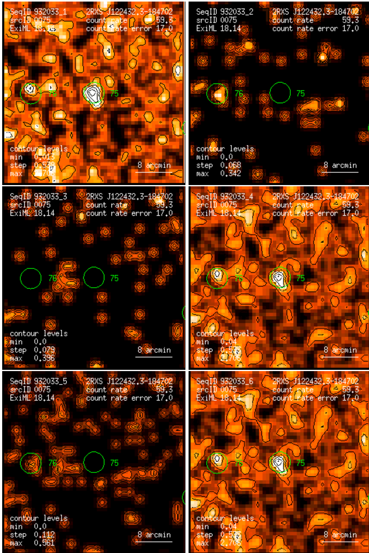
Figure 75: RASS 932033: detection 0075: band rate images, Gaussian filter: (1) PSPC channels 11 – 41, (2) 52 – 90, (3) 91 – 201, (4) 11 – 235, (5) 52 – 201, (6) 11 – 201. Broad band rates in counts/ks. Band rate contour levels in counts/ks/arcmin 2 .
