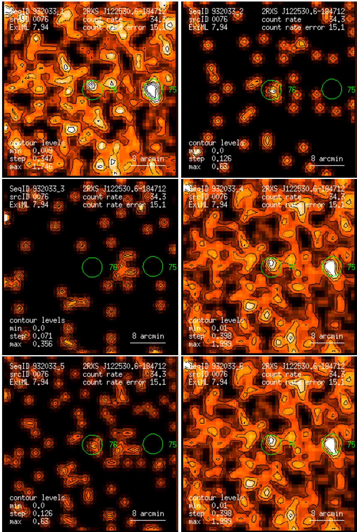
Figure 76: RASS 932033: detection 0076: band rate images, Gaussian filter: (1) PSPC channels 11 – 41, (2) 52 – 90, (3) 91 – 201, (4) 11 – 235, (5) 52 – 201, (6) 11 – 201. Broad band rates in counts/ks. Band rate contour levels in counts/ks/arcmin 2 .
