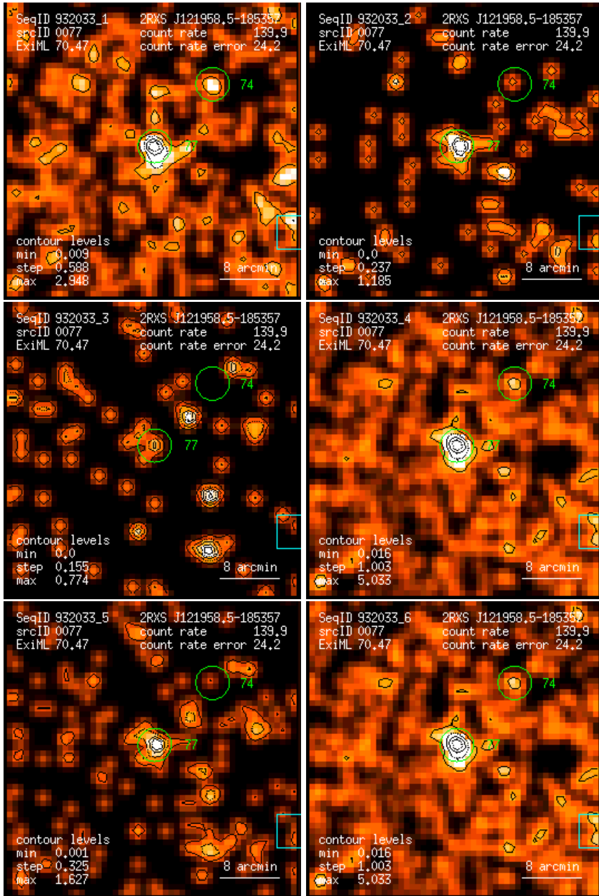
Figure 77: RASS 932033: detection 0077: band rate images, Gaussian filter: (1) PSPC channels 11 – 41, (2) 52 – 90, (3) 91 – 201, (4) 11 – 235, (5) 52 – 201, (6) 11 – 201. Broad band rates in counts/ks. Band rate contour levels in counts/ks/arcmin 2 .
