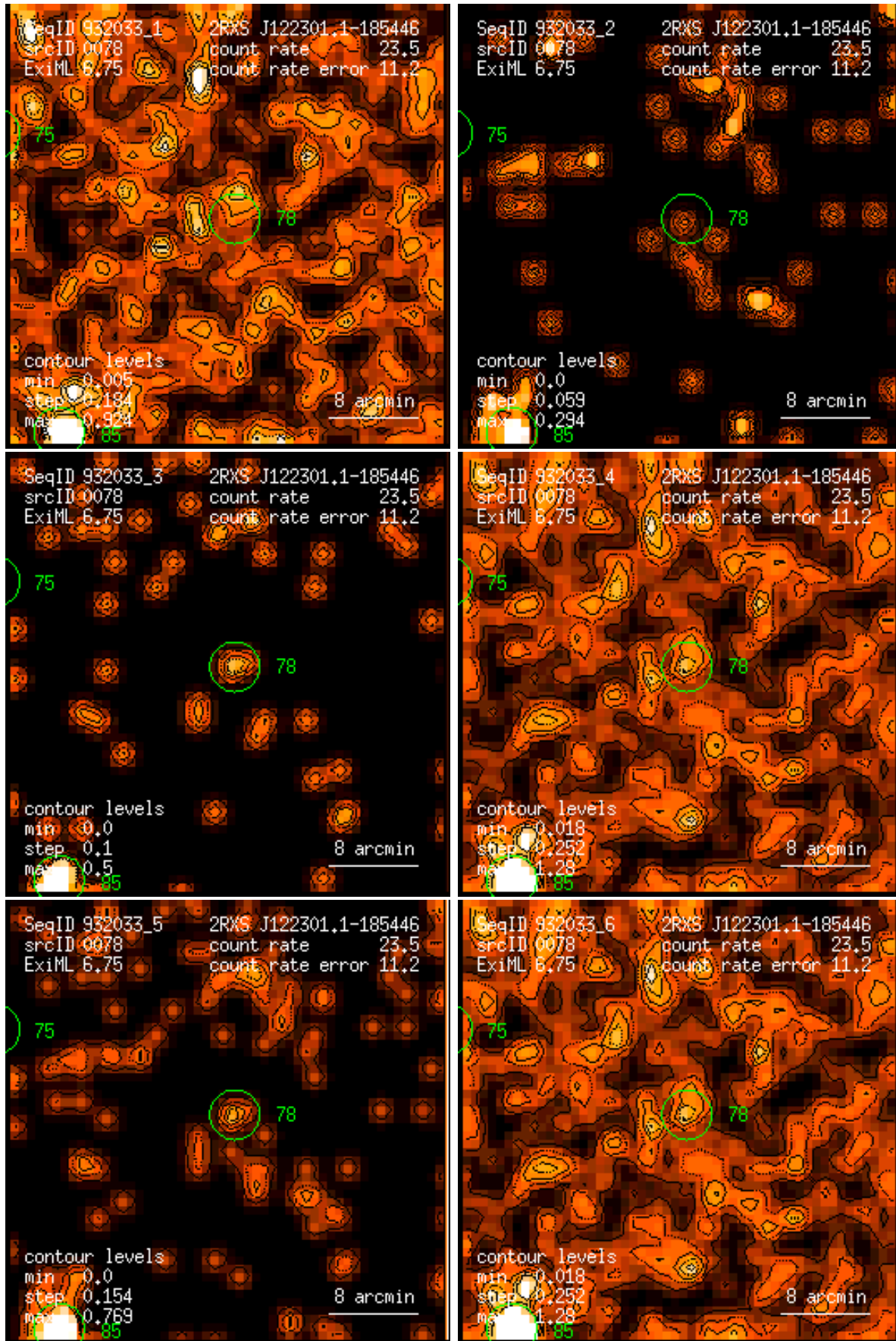
Figure 78: RASS 932033: detection 0078: band rate images, Gaussian filter: (1) PSPC channels 11 – 41, (2) 52 – 90, (3) 91 – 201, (4) 11 – 235, (5) 52 – 201, (6) 11 – 201. Broad band rates in counts/ks. Band rate contour levels in counts/ks/arcmin 2 .
