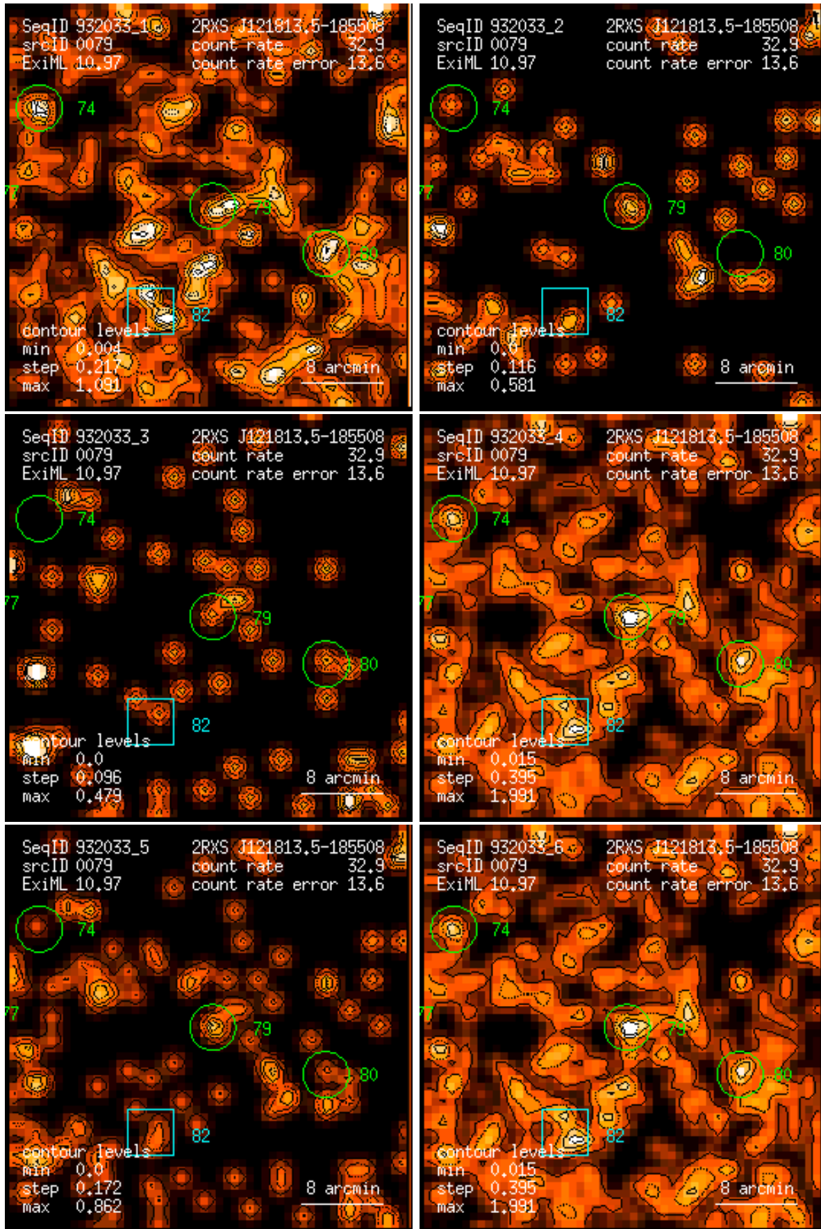
Figure 79: RASS 932033: detection 0079: band rate images, Gaussian filter: (1) PSPC channels 11 – 41, (2) 52 – 90, (3) 91 – 201, (4) 11 – 235, (5) 52 – 201, (6) 11 – 201. Broad band rates in counts/ks. Band rate contour levels in counts/ks/arcmin 2 .
