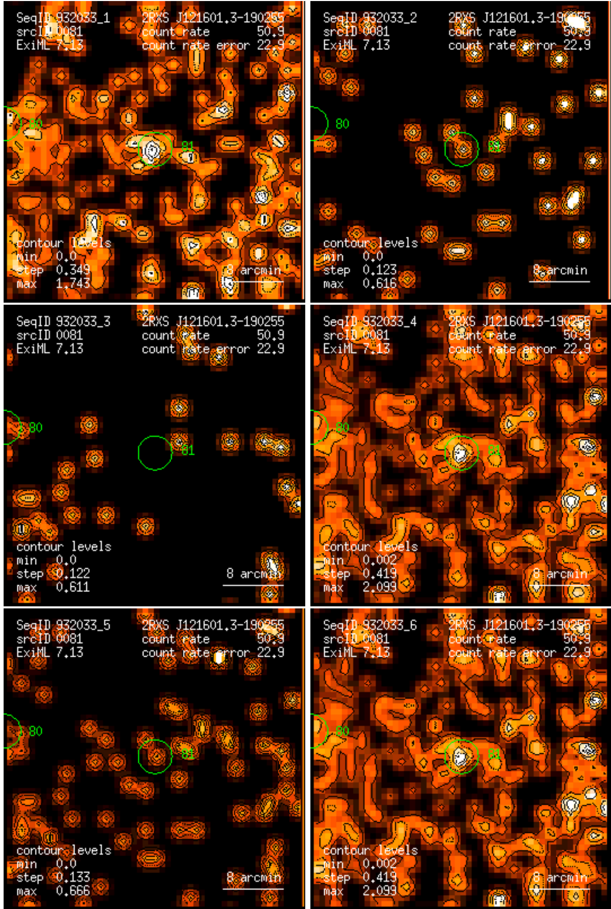
Figure 81: RASS 932033: detection 0081: band rate images, Gaussian filter: (1) PSPC channels 11 – 41, (2) 52 – 90, (3) 91 – 201, (4) 11 – 235, (5) 52 – 201, (6) 11 – 201. Broad band rates in counts/ks. Band rate contour levels in counts/ks/arcmin 2 .
