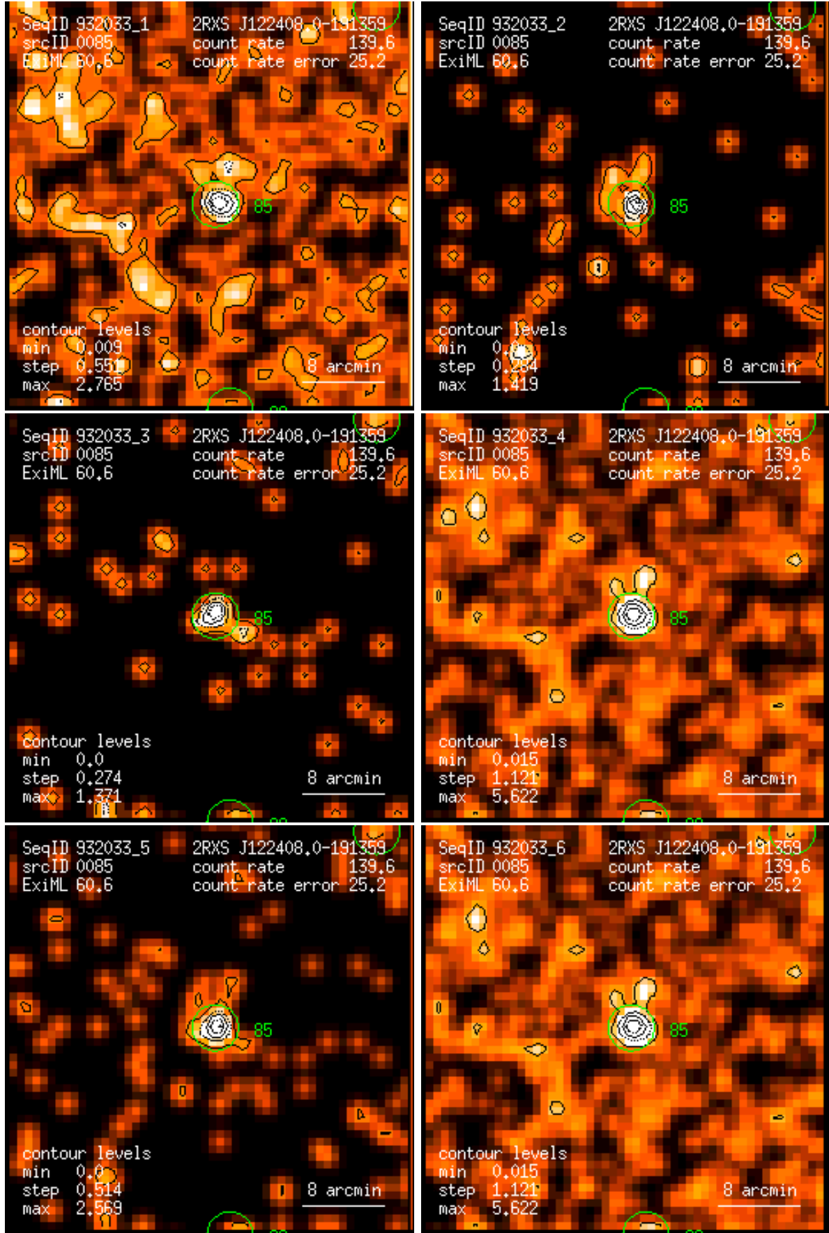
Figure 85: RASS 932033: detection 0085: band rate images, Gaussian filter: (1) PSPC channels 11 – 41, (2) 52 – 90, (3) 91 – 201, (4) 11 – 235, (5) 52 – 201, (6) 11 – 201. Broad band rates in counts/ks. Band rate contour levels in counts/ks/arcmin 2 .
