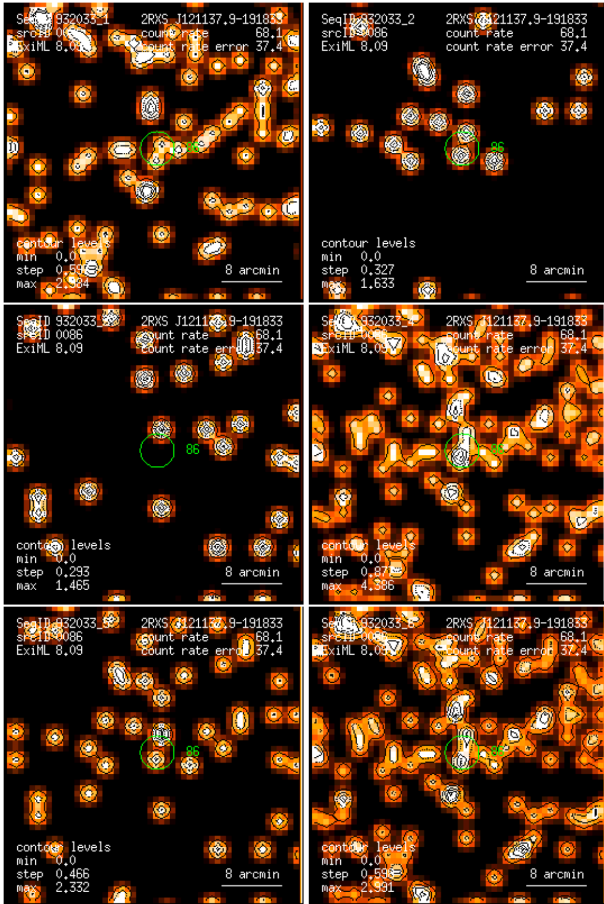
Figure 86: RASS 932033: detection 0086: band rate images, Gaussian filter: (1) PSPC channels 11 – 41, (2) 52 – 90, (3) 91 – 201, (4) 11 – 235, (5) 52 – 201, (6) 11 – 201. Broad band rates in counts/ks. Band rate contour levels in counts/ks/arcmin 2 .
