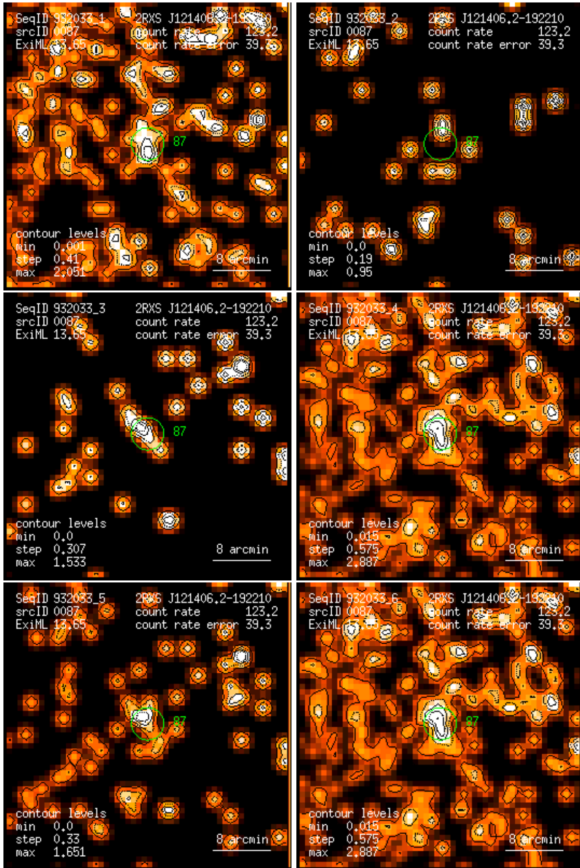
Figure 87: RASS 932033: detection 0087: band rate images, Gaussian filter: (1) PSPC channels 11 – 41, (2) 52 – 90, (3) 91 – 201, (4) 11 – 235, (5) 52 – 201, (6) 11 – 201. Broad band rates in counts/ks. Band rate contour levels in counts/ks/arcmin 2 .
