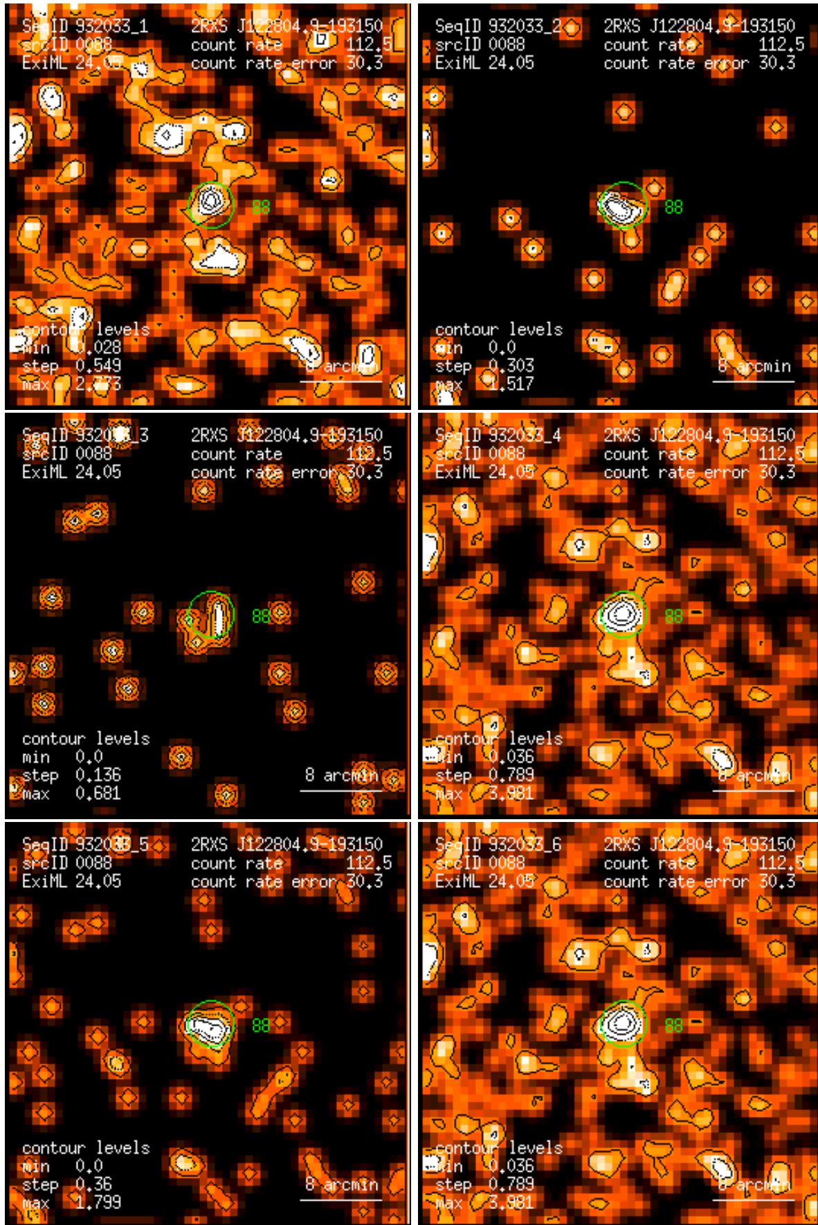
Figure 88: RASS 932033: detection 0088: band rate images, Gaussian filter: (1) PSPC channels 11 – 41, (2) 52 – 90, (3) 91 – 201, (4) 11 – 235, (5) 52 – 201, (6) 11 – 201. Broad band rates in counts/ks. Band rate contour levels in counts/ks/arcmin 2 .
