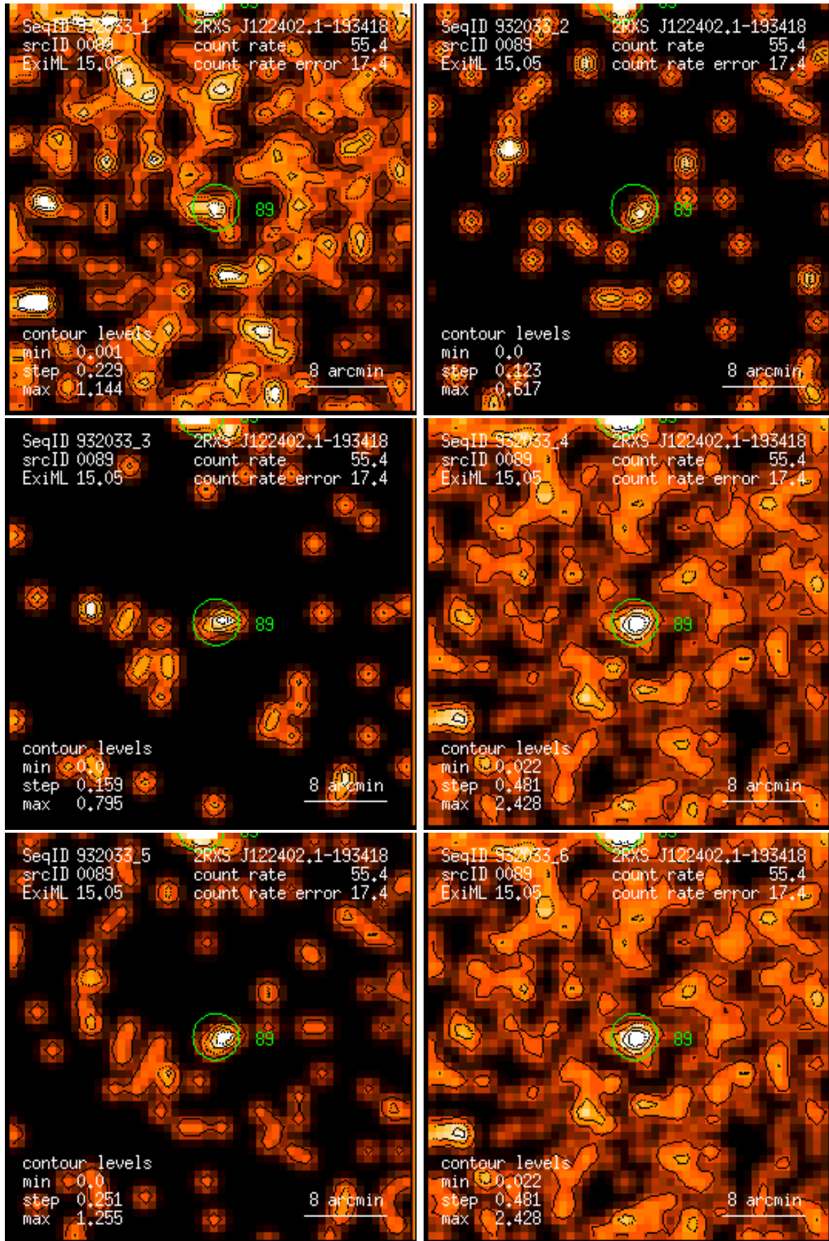
Figure 89: RASS 932033: detection 0089: band rate images, Gaussian filter: (1) PSPC channels 11 – 41, (2) 52 – 90, (3) 91 – 201, (4) 11 – 235, (5) 52 – 201, (6) 11 – 201. Broad band rates in counts/ks. Band rate contour levels in counts/ks/arcmin 2 .
