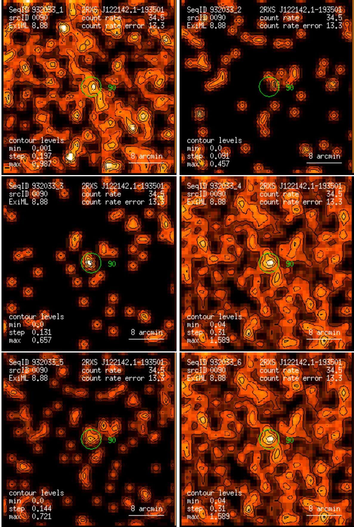
Figure 90: RASS 932033: detection 0090: band rate images, Gaussian filter: (1) PSPC channels 11 – 41, (2) 52 – 90, (3) 91 – 201, (4) 11 – 235, (5) 52 – 201, (6) 11 – 201. Broad band rates in counts/ks. Band rate contour levels in counts/ks/arcmin 2 .
