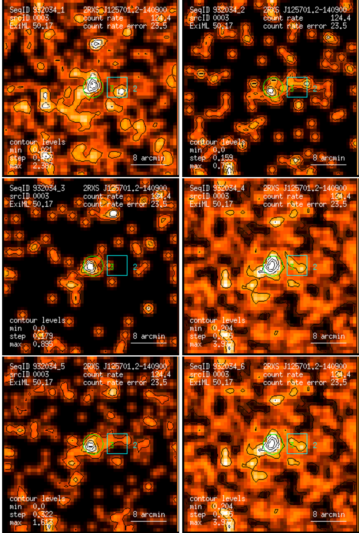
Figure 3: RASS 932034: detection 0003: band rate images, Gaussian filter: (1) PSPC channels 11 – 41, (2) 52 – 90, (3) 91 – 201, (4) 11 – 235, (5) 52 – 201, (6) 11 – 201. Broad band rates in counts/ks. Band rate contour levels in counts/ks/arcmin 2 .
