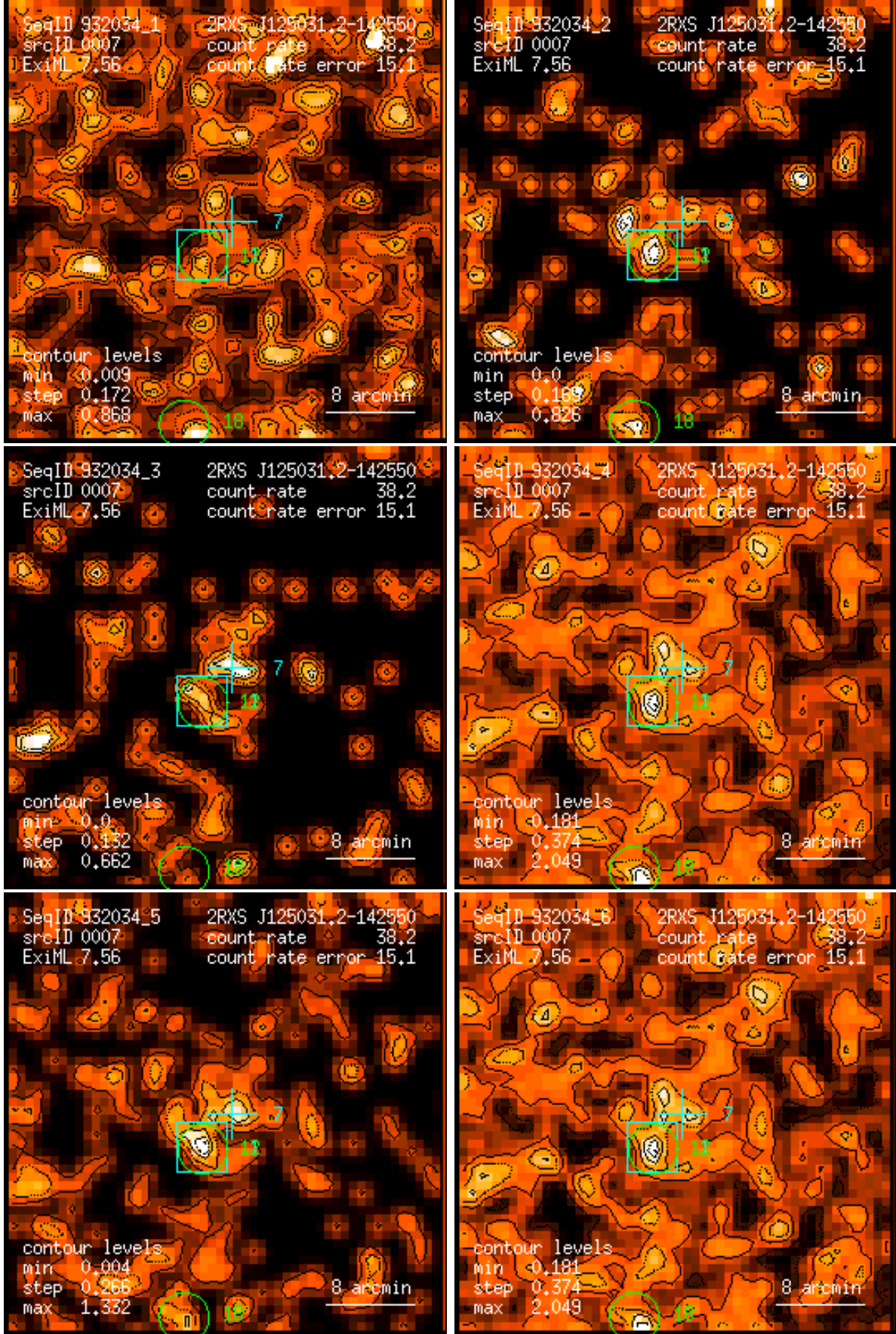
Figure 7: RASS 932034: detection 0007: band rate images, Gaussian filter: (1) PSPC channels 11 – 41, (2) 52 – 90, (3) 91 – 201, (4) 11 – 235, (5) 52 – 201, (6) 11 – 201. Broad band rates in counts/ks. Band rate contour levels in counts/ks/arcmin 2 .
