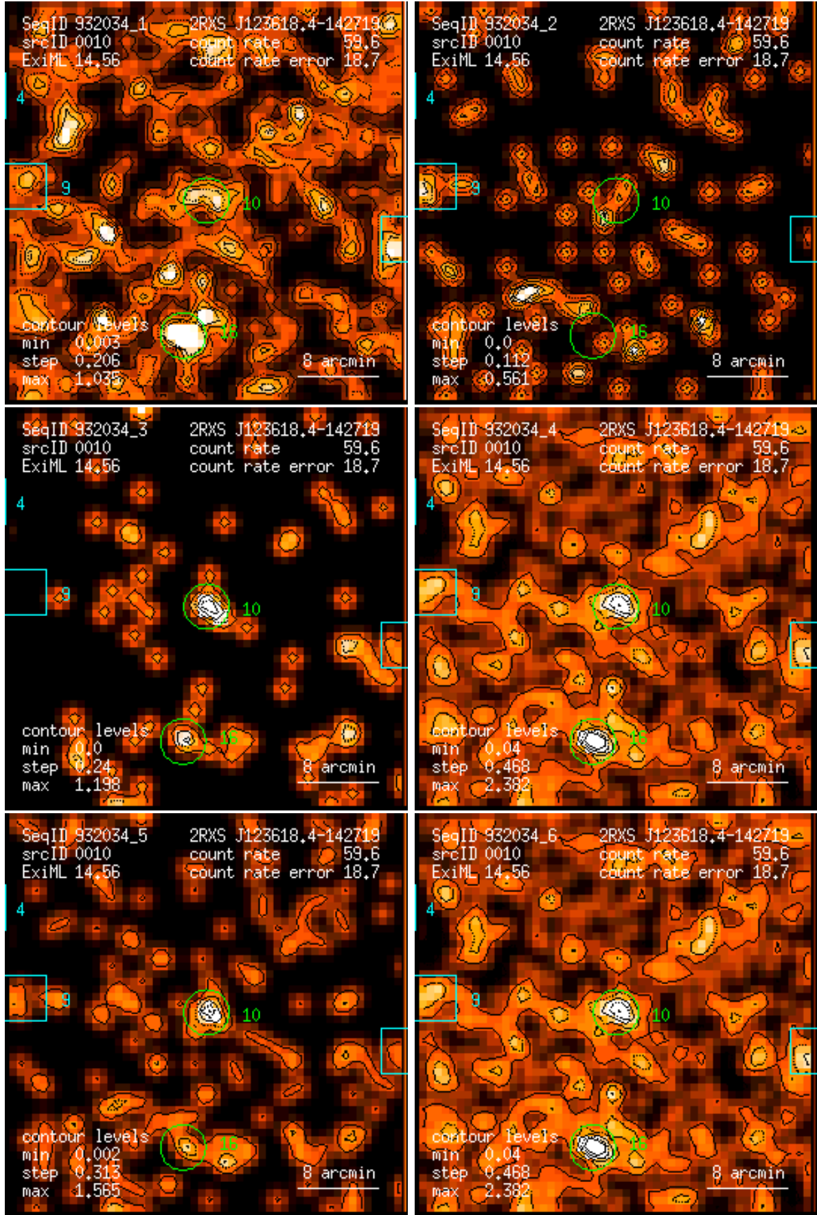
Figure 10: RASS 932034: detection 0010: band rate images, Gaussian filter: (1) PSPC channels 11 – 41, (2) 52 – 90, (3) 91 – 201, (4) 11 – 235, (5) 52 – 201, (6) 11 – 201. Broad band rates in counts/ks. Band rate contour levels in counts/ks/arcmin 2 .
