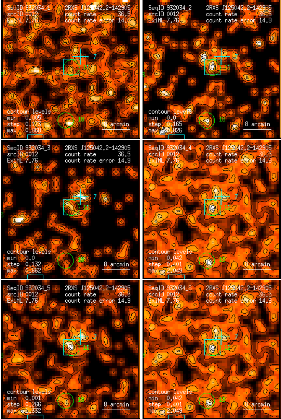
Figure 12: RASS 932034: detection 0012: band rate images, Gaussian filter: (1) PSPC channels 11 – 41, (2) 52 – 90, (3) 91 – 201, (4) 11 – 235, (5) 52 – 201, (6) 11 – 201. Broad band rates in counts/ks. Band rate contour levels in counts/ks/arcmin 2 .
