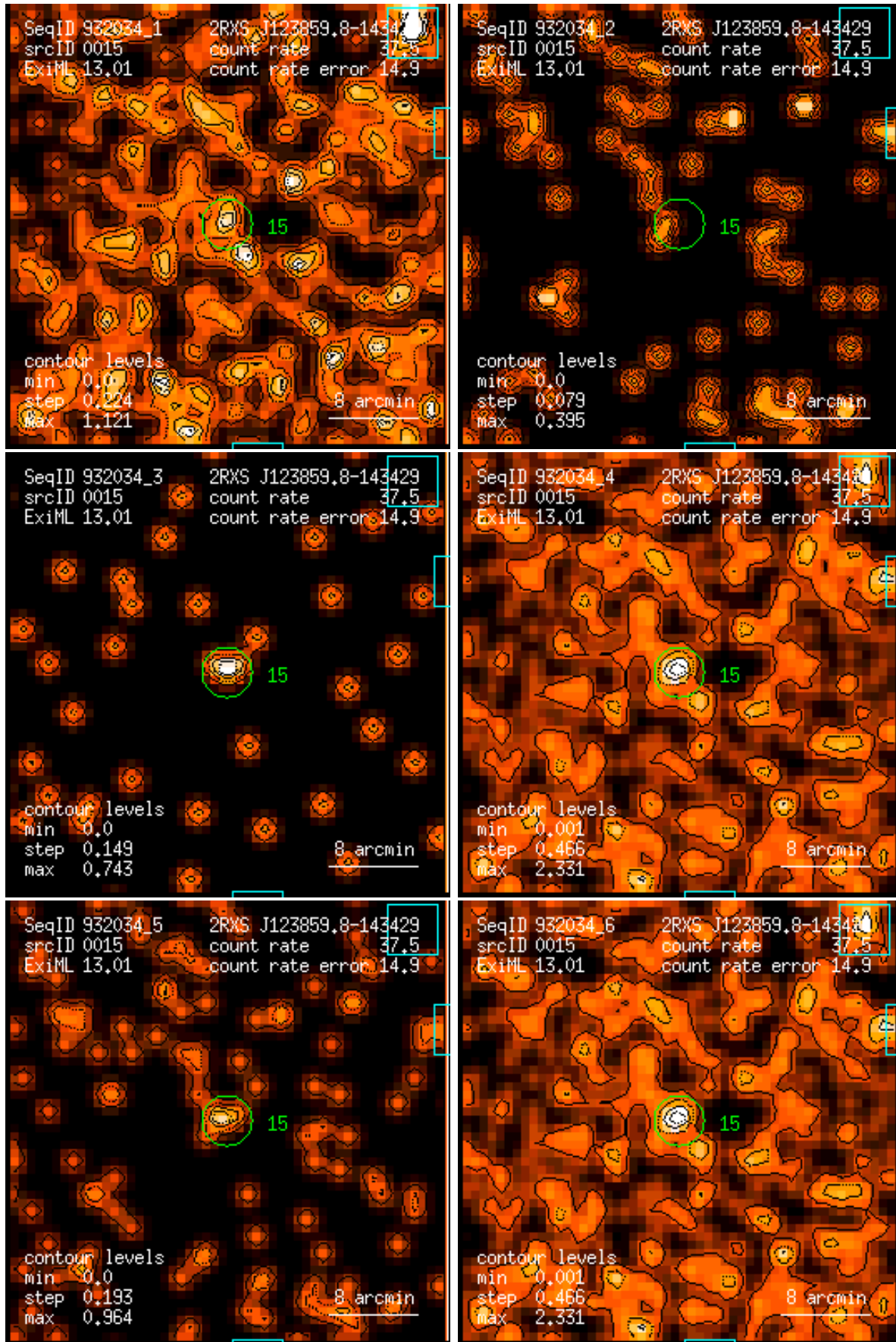
Figure 15: RASS 932034: detection 0015: band rate images, Gaussian filter: (1) PSPC channels 11 – 41, (2) 52 – 90, (3) 91 – 201, (4) 11 – 235, (5) 52 – 201, (6) 11 – 201. Broad band rates in counts/ks. Band rate contour levels in counts/ks/arcmin 2 .
