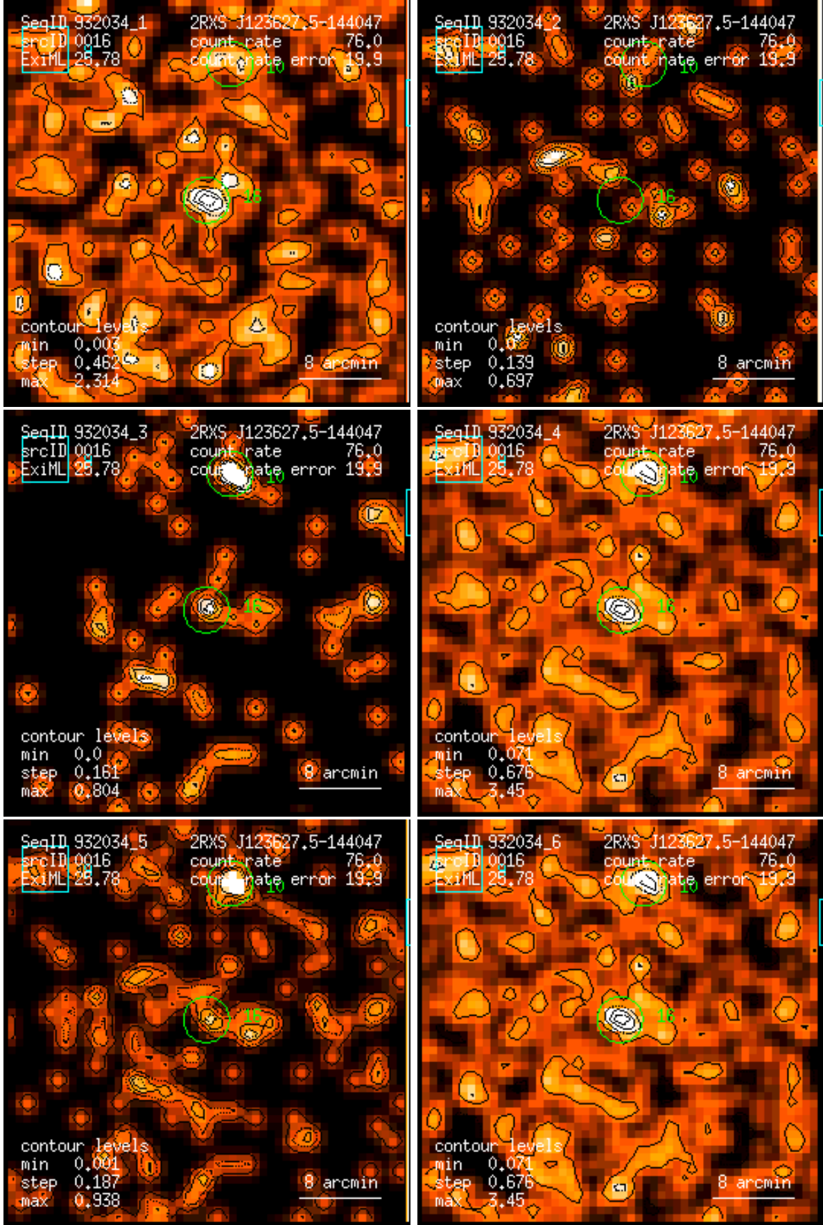
Figure 16: RASS 932034: detection 0016: band rate images, Gaussian filter: (1) PSPC channels 11 – 41, (2) 52 – 90, (3) 91 – 201, (4) 11 – 235, (5) 52 – 201, (6) 11 – 201. Broad band rates in counts/ks. Band rate contour levels in counts/ks/arcmin 2 .
